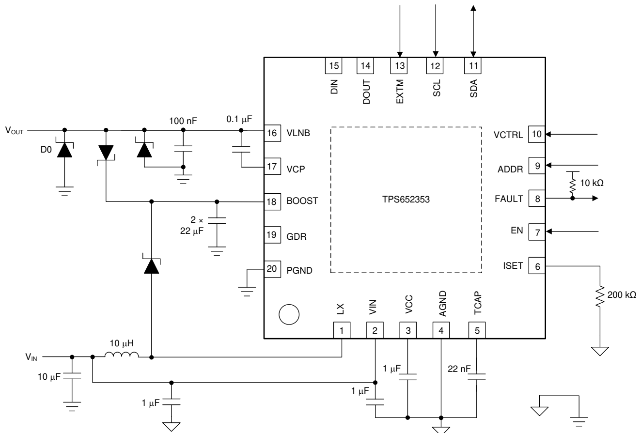
8-1. Application for DiSEqc1.x Support
