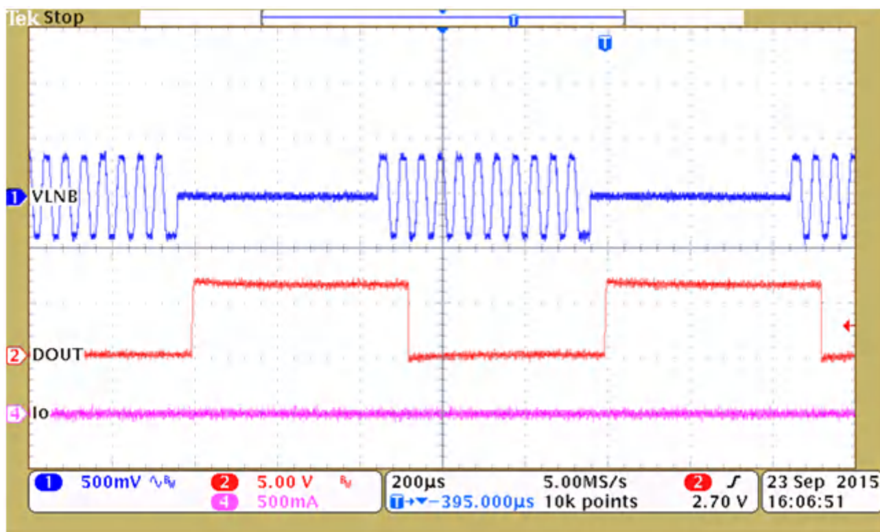
8-21. DOUT Tone Detection Output
