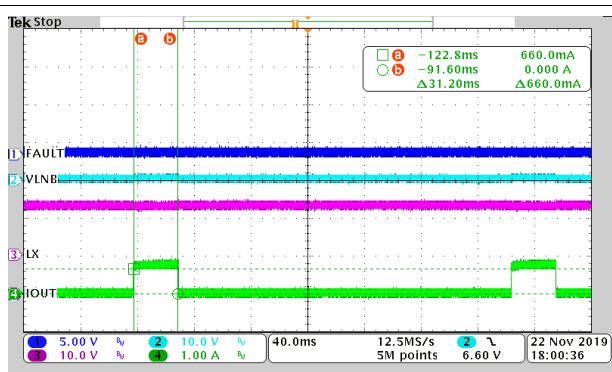
Figure 8-19. Hiccup Operation at R_{SET} = 200\text{ k}\Omega
