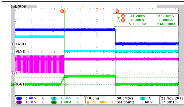
Figure 8-18. Current Limit Operation at R_{SET} = 200\text{ k}\Omega
