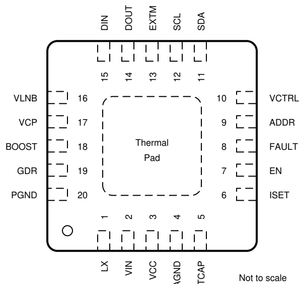
図 5-1. RUK Package. 20-Pin WQFN With Exposed Thermal Pad. Top View.
