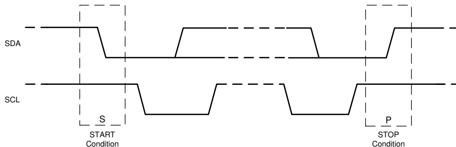
图 6-5. Start and Stop Sequences
