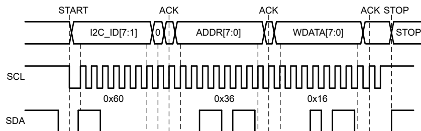
図 6-8. I 2 C Write Cycle without CRC
