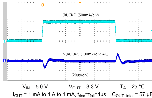
图 5-4. BUCK2 Load-step response - Low Bandwidth, forced PWM
