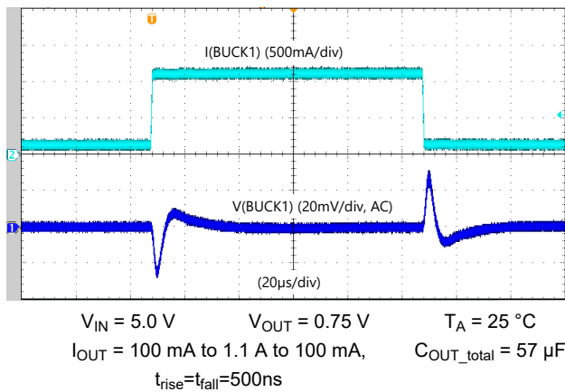
图 5-3. BUCK1 Load-step response - High Bandwidth, forced PWM
