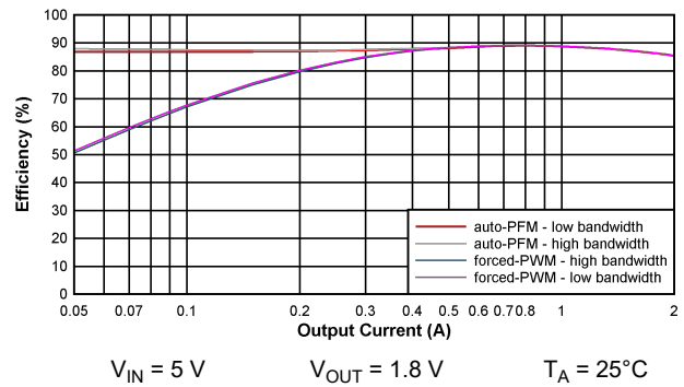
图 5-2. Efficiency BUCK23
