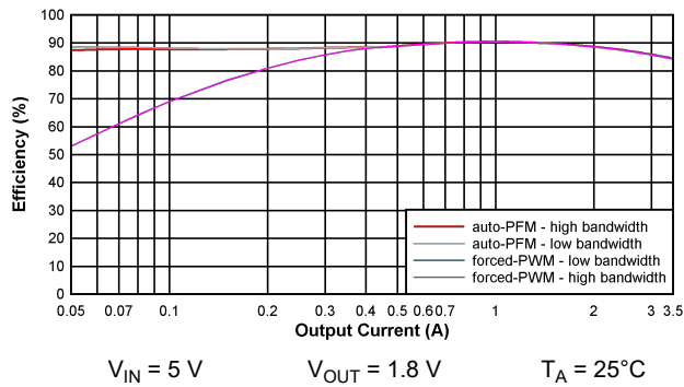
图 5-1. Efficiency BUCK1
