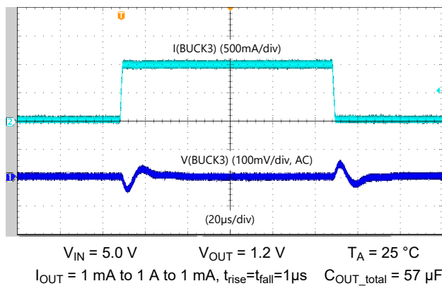
图 5-5. BUCK3 Load-step response - Low Bandwidth, forced PWM
