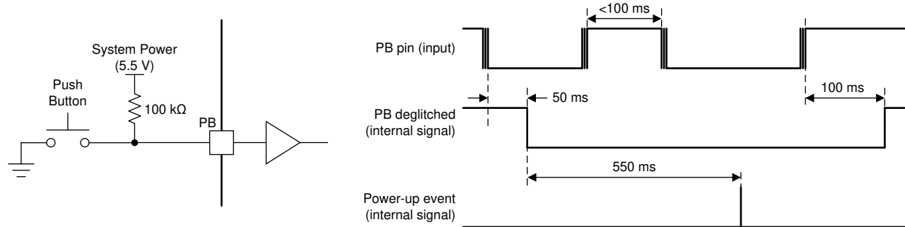
FIG 7-18. Left: Typical PB Input Circuit Right: Push-Button Input (PB) Deglitch and Power-Up Timing
