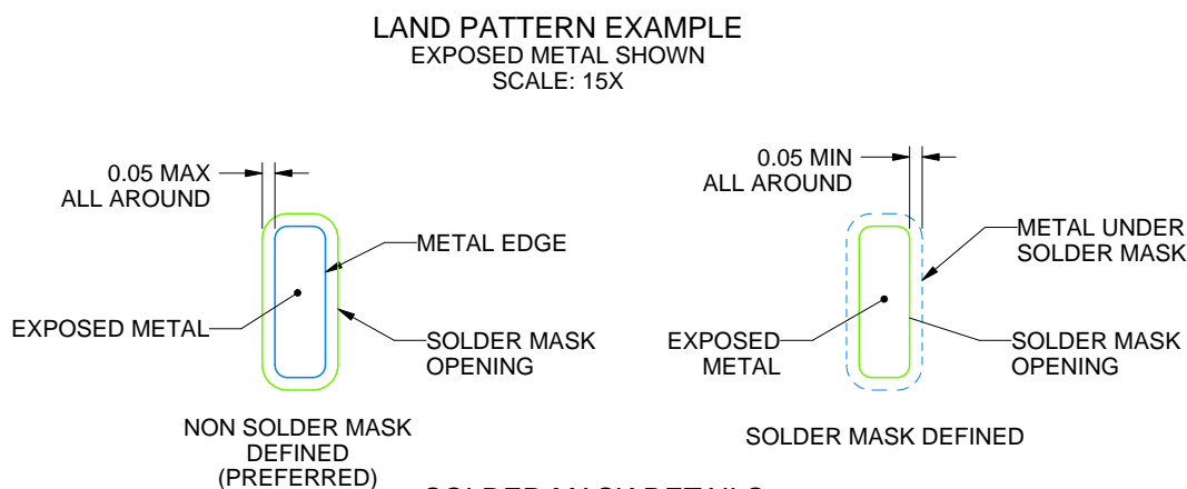
SOLDER MASK DETAILS
