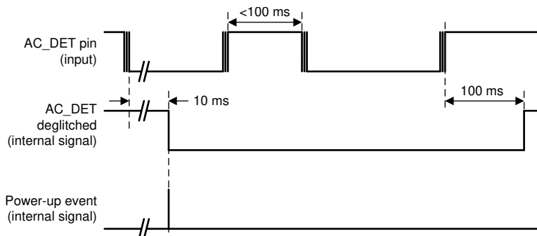
FIG 7-29. AC_DET Input Deglitch and Power-Up Timing (Portable Systems)
