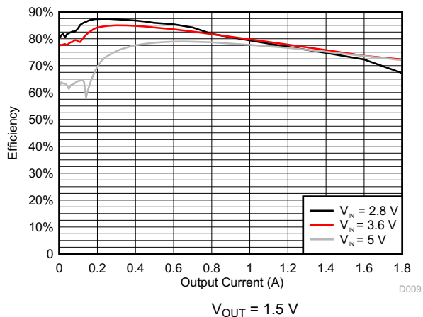
8-5. DCDC3 Efficiency
