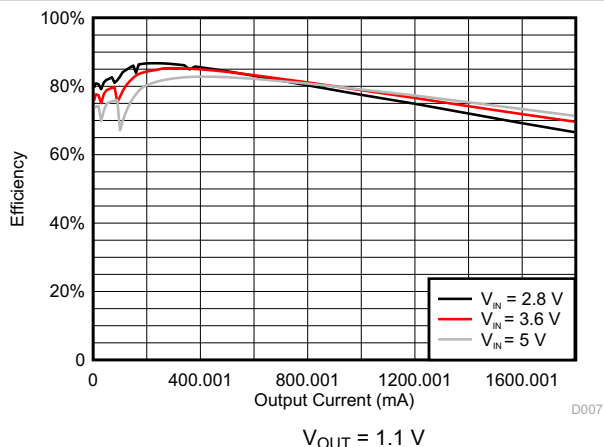
8-3. DCDC1/DCDC2 Efficiency
