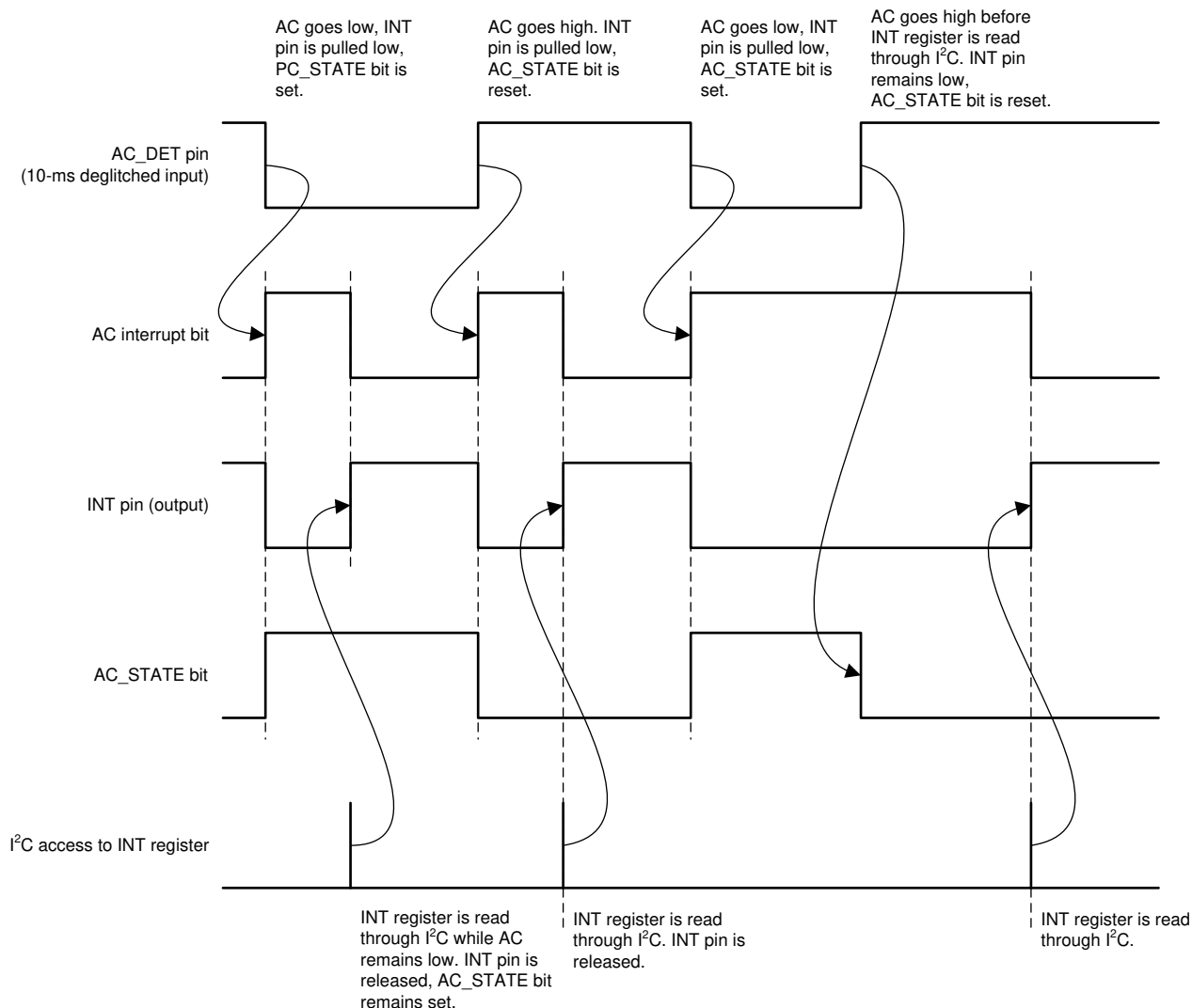
图 7-30. AC_STATE Pin
