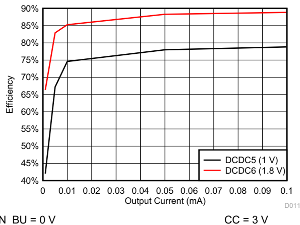
8-7. DCDC5/DCDC6 Efficiency
