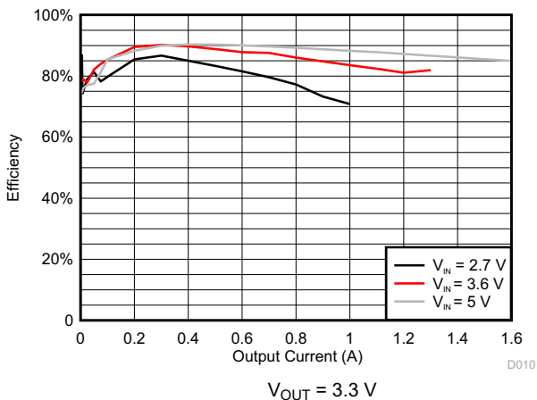
8-6. DCDC4 Efficiency
