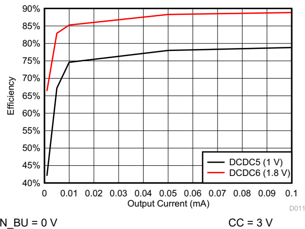
8-8. DCDC5/DCDC6 Efficiency
