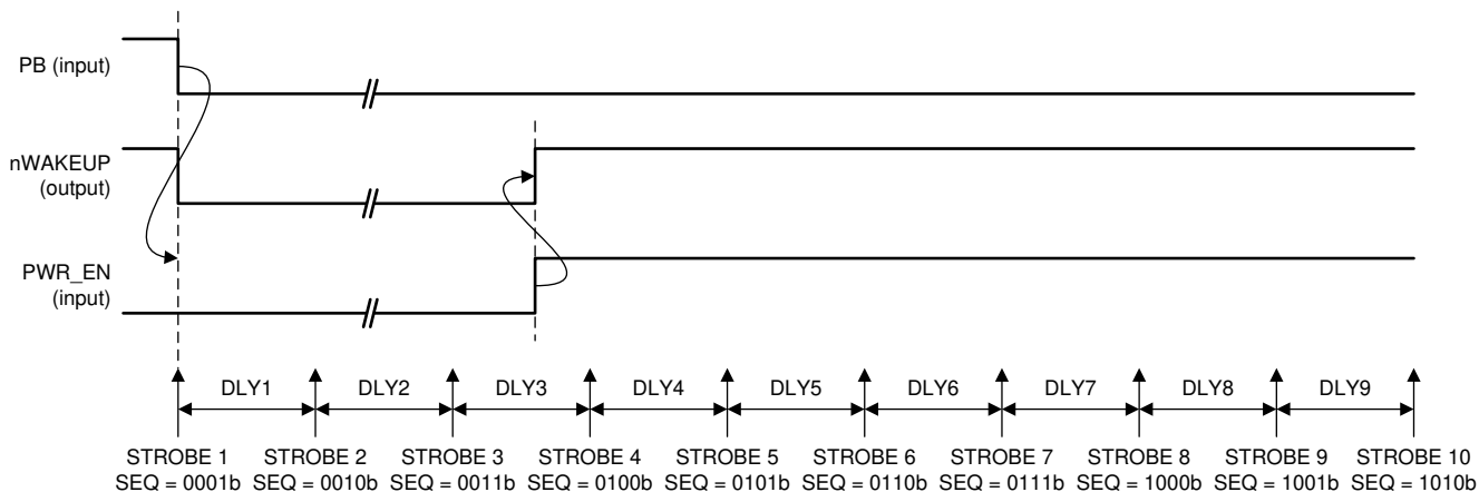
Figure 7-1. Power-Up Sequences from OFF or SUSPEND State; PB is Power-Up Event
