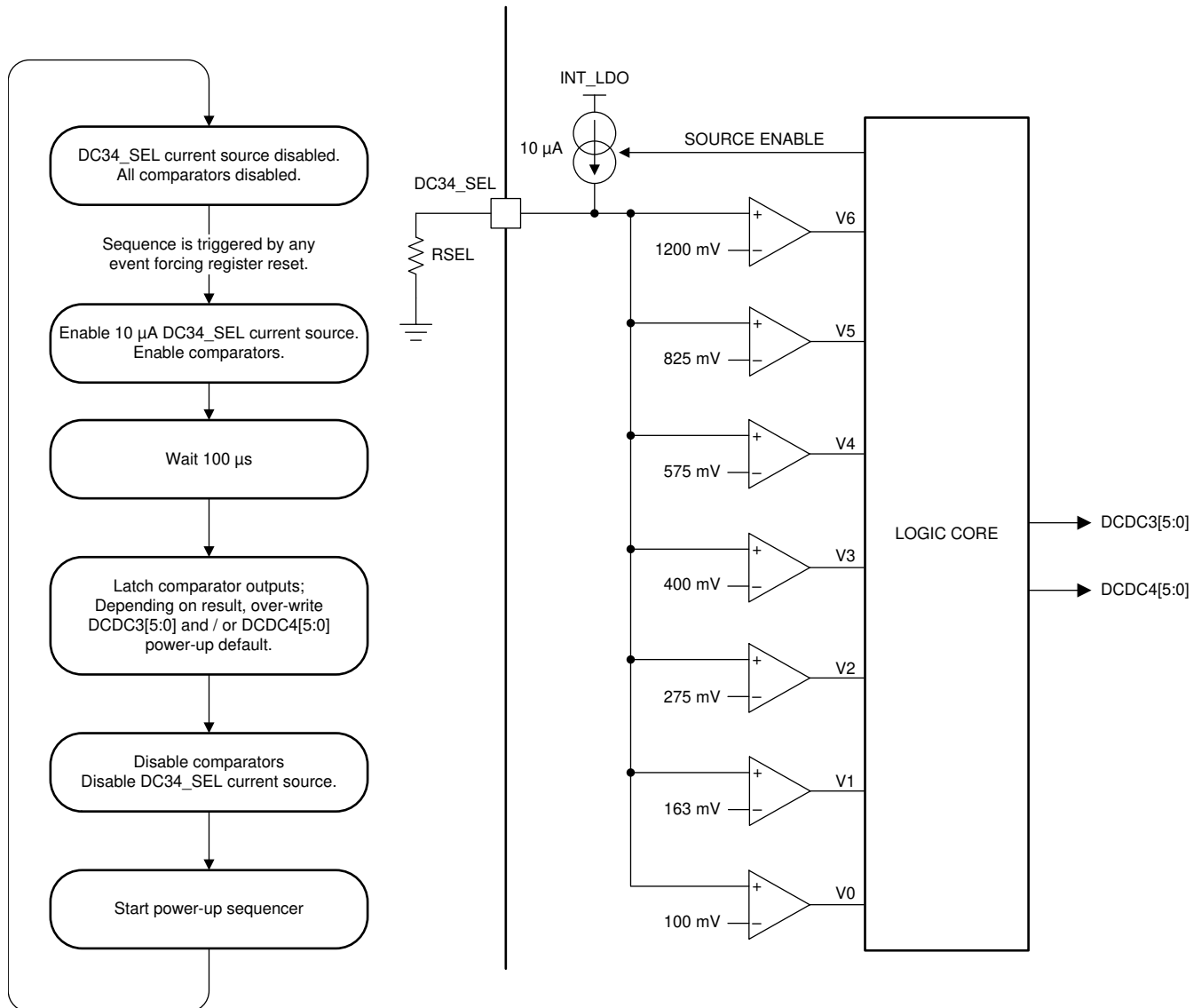
图 7-21. Left: Flow Chart for Selecting DCDC Power-Up Default Voltage Right: Comparator Circuit
