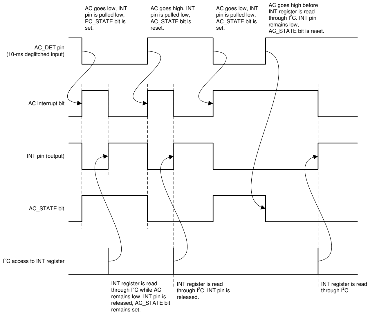
图 7-29. AC_STATE Pin
