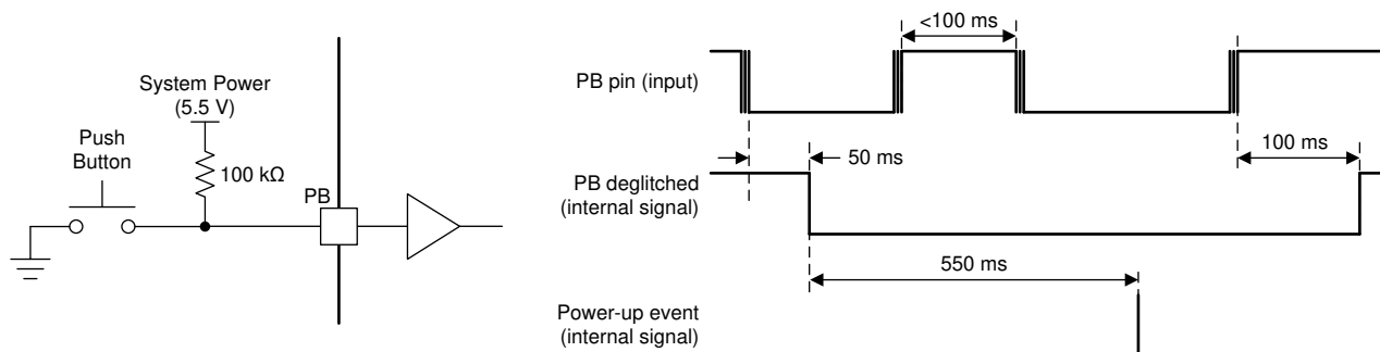
图 7-25. Left: Typical PB Input Circuit Right: Push-Button Input (PB) Deglitch and Power-Up Timing
