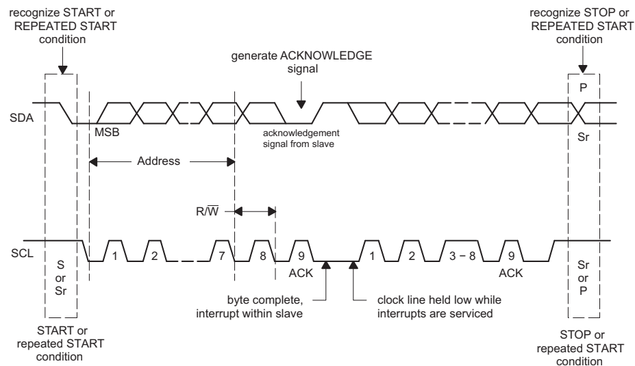
Figure 6-20. Bus Protocol
