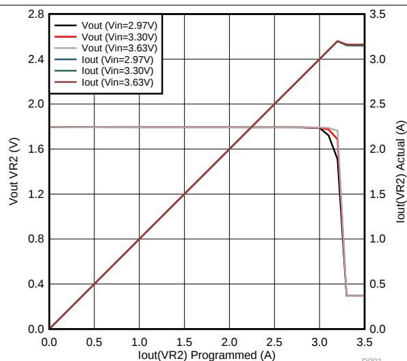
Figure 5-17. VR2 Current Limit: Vout and Iout vs Load, Non-NVDC
