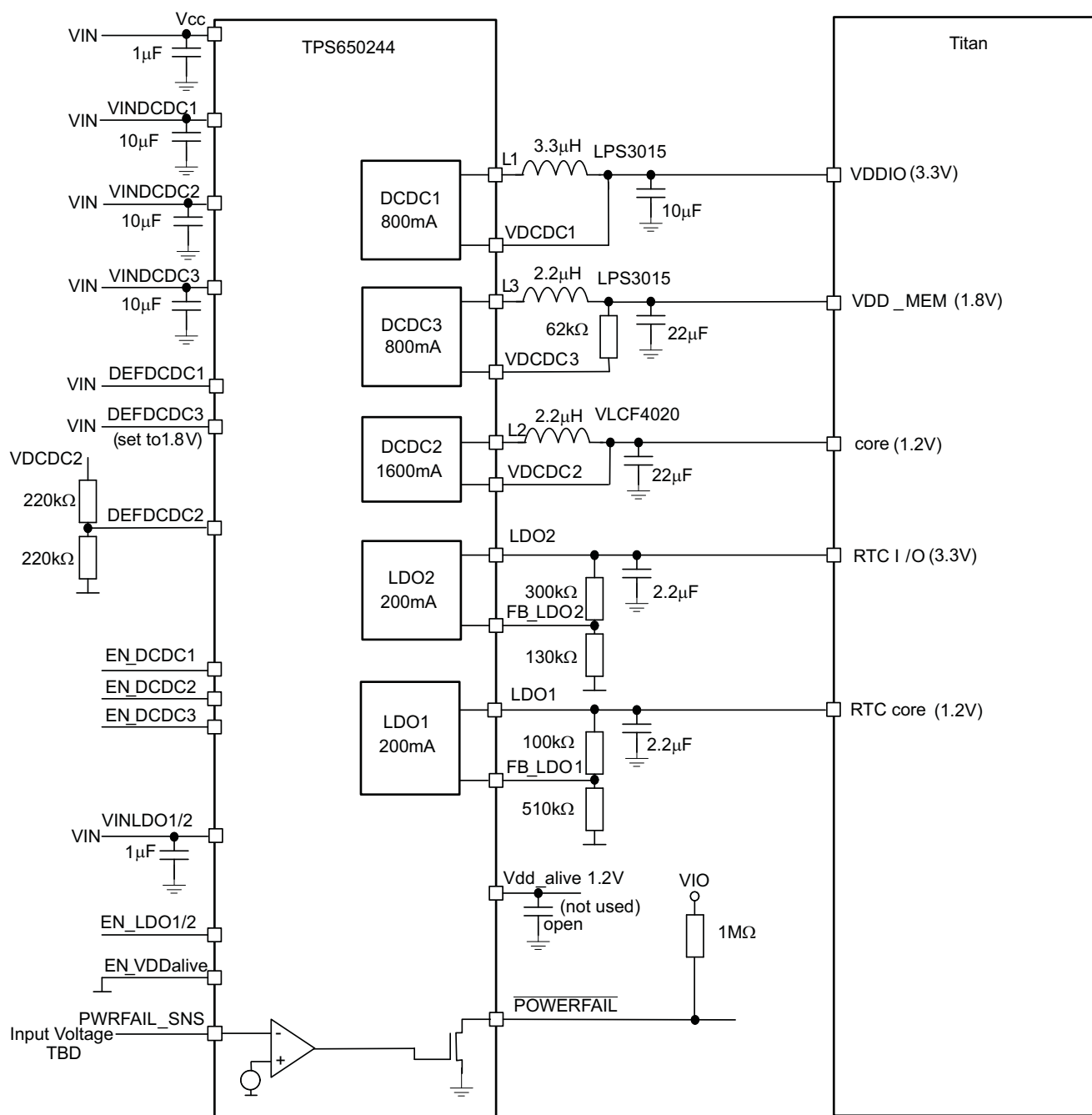
Figure 18. Titan Processor Configuration
