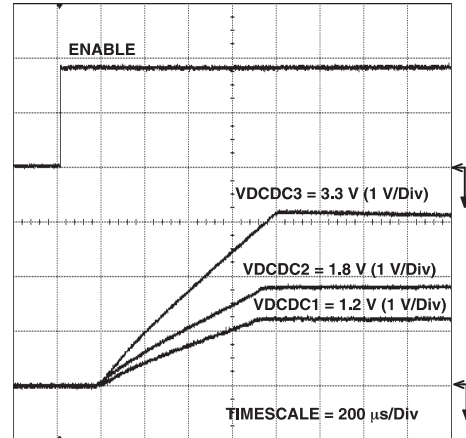
Figure 22. Start-Up VDCDC1, VDCDC2, and VDCDC3
