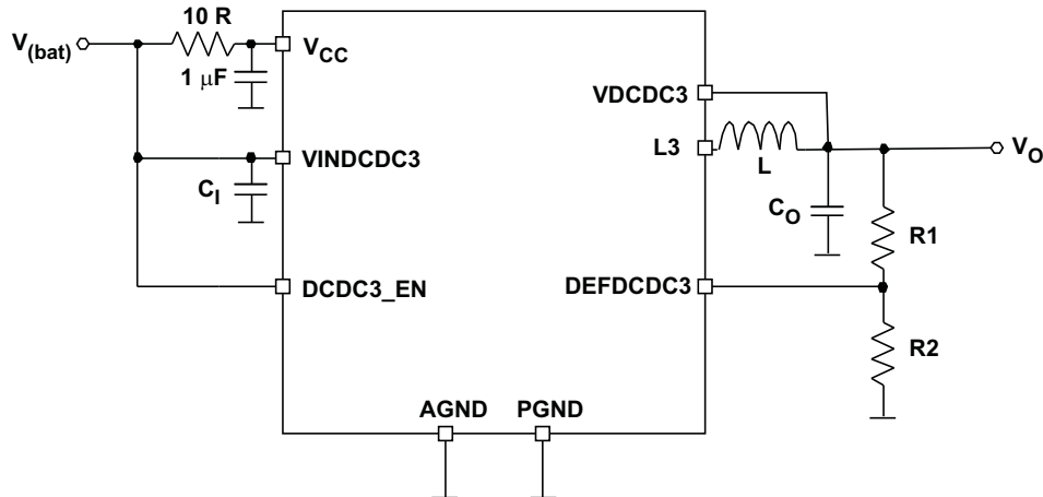
Figure 41. External Resistor Divider
