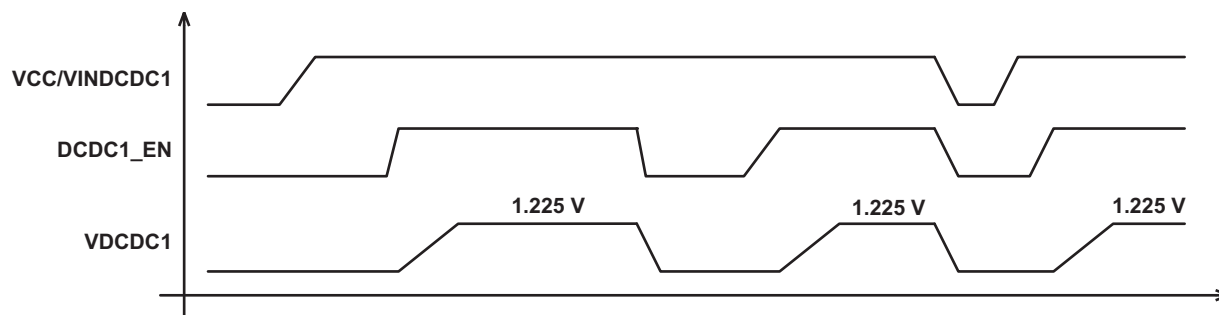
Figure 38. Default DCDC1
