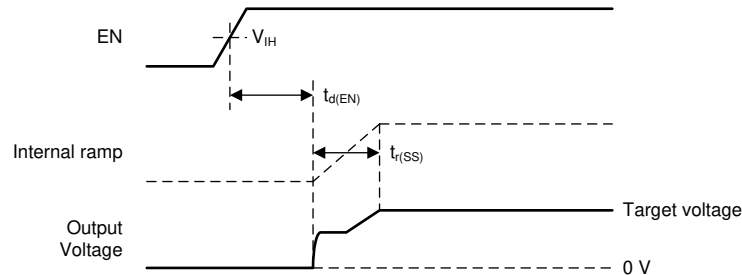
Figure 6-6. Start-Up Behavior
