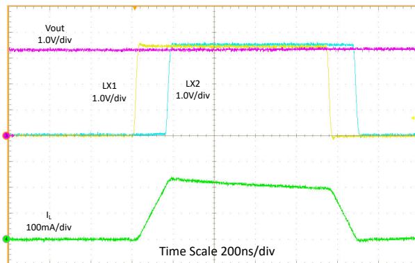
図 7-15. Switching Waveforms, Buck-Boost Operation
