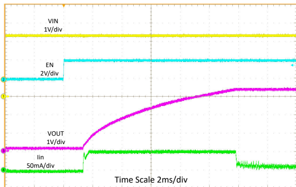
図 7-26. Start-Up with 50-mA ICL
