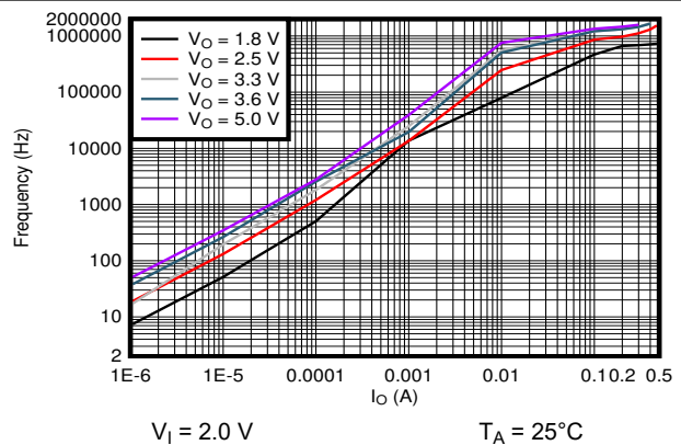
Figure 7-7. Typical Burst Switching Frequency vs Output Current
