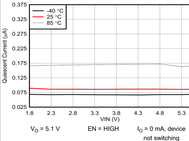
5-2. Quiescent Current into VOUT vs Input Voltage
