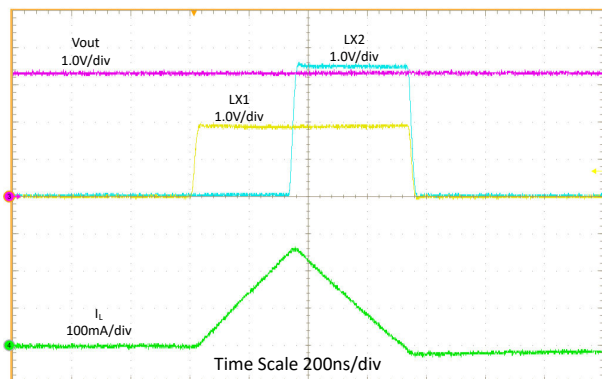
図 7-14. Switching Waveforms, Boost Operation
