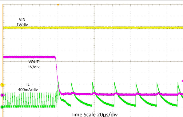
図 7-27. Short Circuit Behavior
