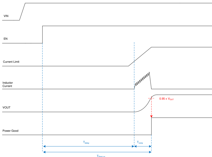
Figure 9-4. Device Start-up Scheme
