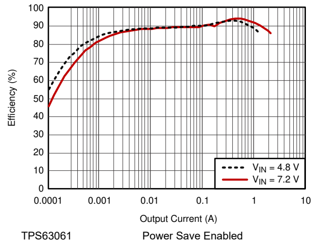
Figure 9-5. Efficiency vs. Output Current
