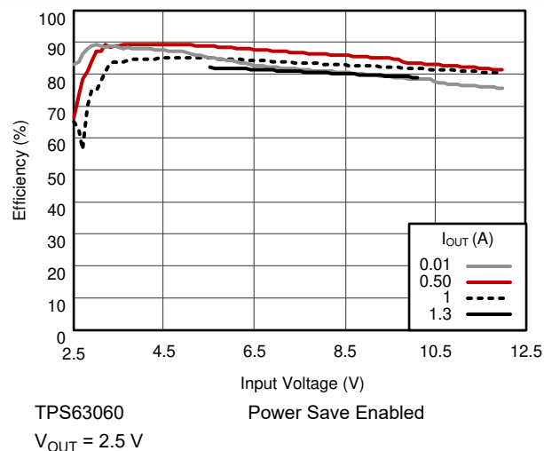
Figure 9-6. Efficiency vs. Input Voltage
