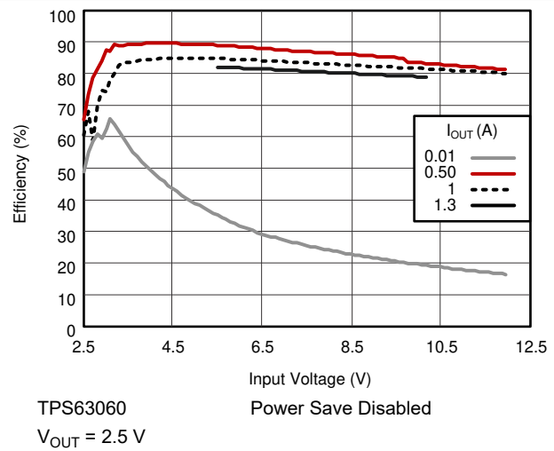
Figure 9-7. Efficiency vs. Input Voltage
