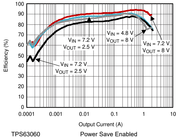
Figure 9-2. Efficiency vs. Output Current
