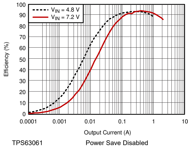
Figure 9-4. Efficiency vs. Output Current
