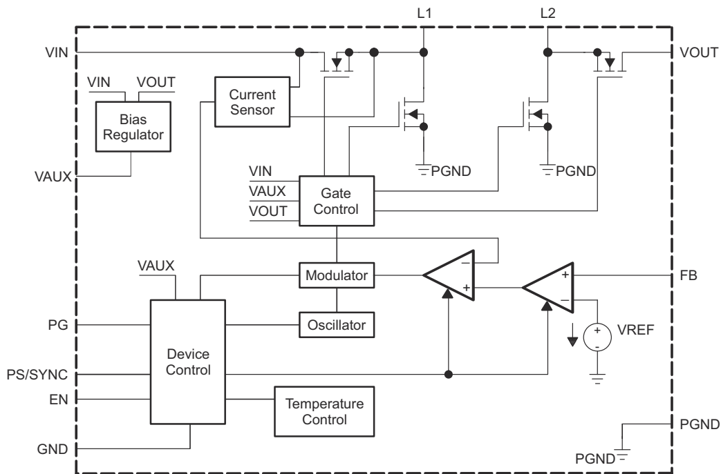
8-1. TPS63060 Adjustable
