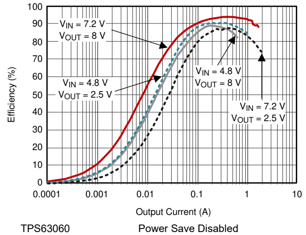
Figure 9-3. Efficiency vs. Output Current
