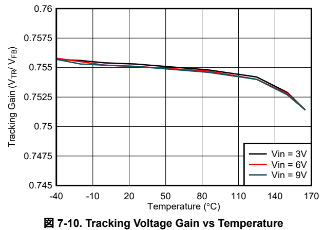
Figure 7-10. Tracking Voltage Gain vs Temperature
