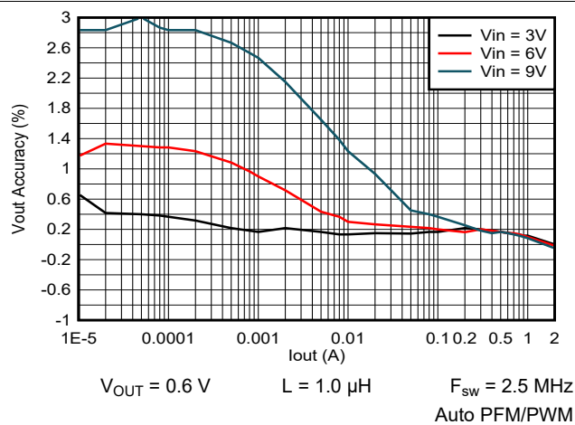
9-31. Output Voltage vs Output Current
