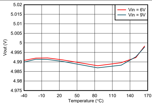
Figure 7-4. Output Voltage Accuracy - VSET Selected
