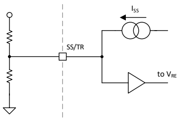
图 8-4. Tracking Operation Simplified Schematic
