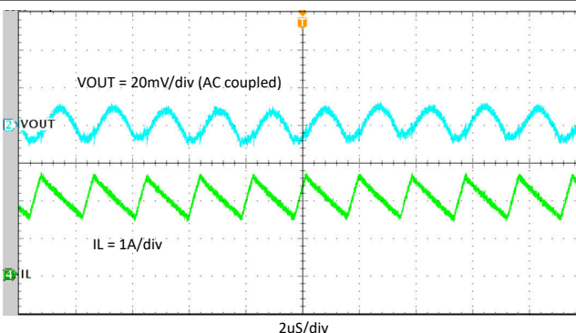
FIG 10-17. Steady State, I_{OUT} = 2 A
