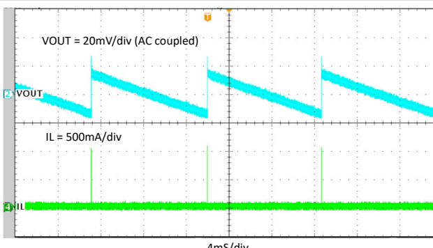
10-13. Steady State, I_{OUT} = 0\text{ A}
