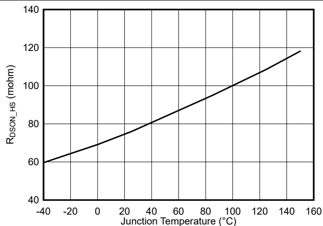
FIG 8-3. High-Side R_{DS(on)} vs Junction Temperature
