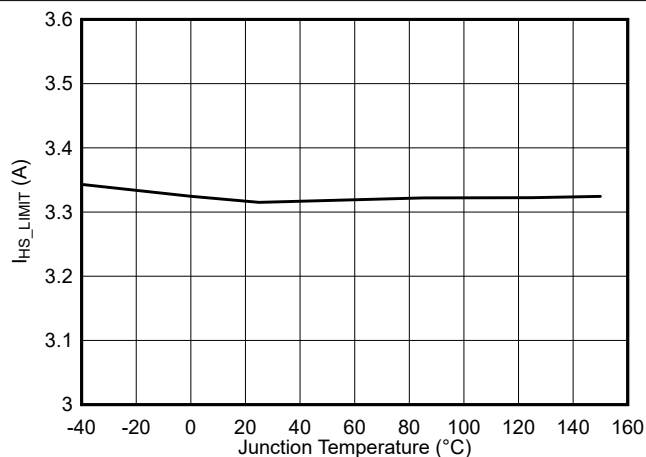
FIG 8-13. TPS62932 High-Side Current Limit vs Junction Temperature
