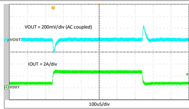
FIG 10-19. Load Transient Response, 0.5 to 2.5 A, Slew Rate = 0.8 A/ \mu S
