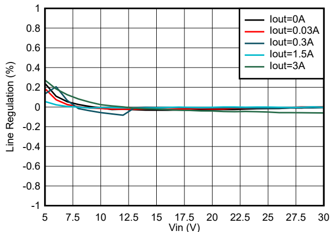
8-30. TPS62933 Line Regulation, V_{OUT} = 3.3\text{ V} , f_{SW} = 500\text{ kHz}
