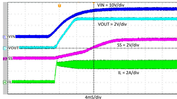
10-9. Start-Up Relative to V_{IN} , I_{OUT} = 3\text{ A}
