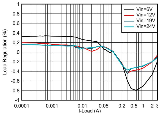
8-29. TPS62933O Load Regulation, V_{OUT} = 5\text{ V} , f_{SW} = 500\text{ kHz}
