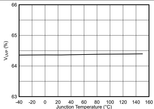
FIG 8-16. UVP Threshold vs Junction Temperature
