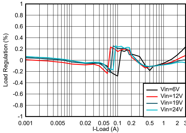
8-25. TPS62933 Load Regulation, V_{OUT} = 3.3\text{ V} , f_{SW} = 1200\text{ kHz}
