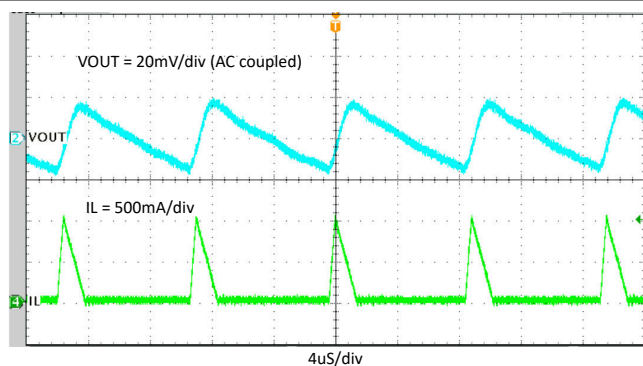
FIG 10-14. Steady State, I_{OUT} = 0.1 A
