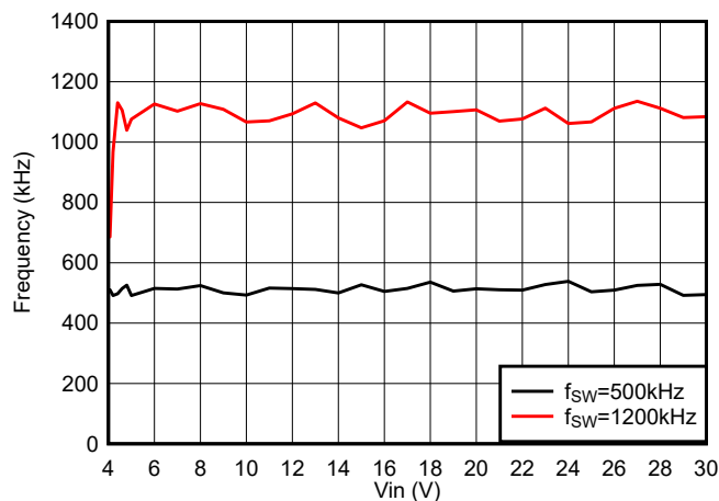
FIG 8-37. TPS62933 Switching Frequency vs V_{IN} , V_{OUT} = 3.3\text{ V} , I_{OUT} = 3\text{ A}
