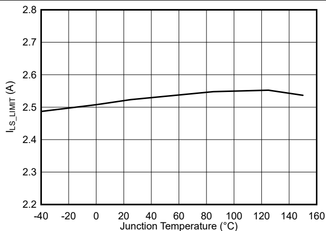
FIG 8-14. TPS62932 Low-Side Current Limit vs Junction Temperature
