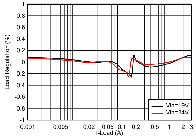
8-26. TPS62933 Load Regulation, V_{OUT} = 12\text{ V} , f_{SW} = 500\text{ kHz}
