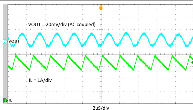
FIG 10-18. Steady State, I_{OUT} = 3 A
