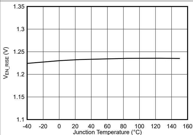
FIG 8-6. Enable Threshold vs Junction Temperature
