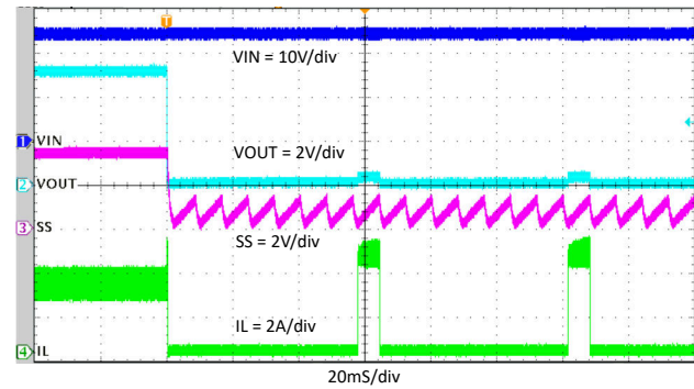
10-21. V_{OUT} Hard Short Protection
