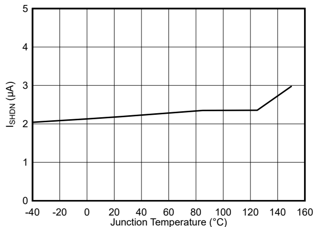
FIG 8-2. Shutdown Current vs Junction Temperature
