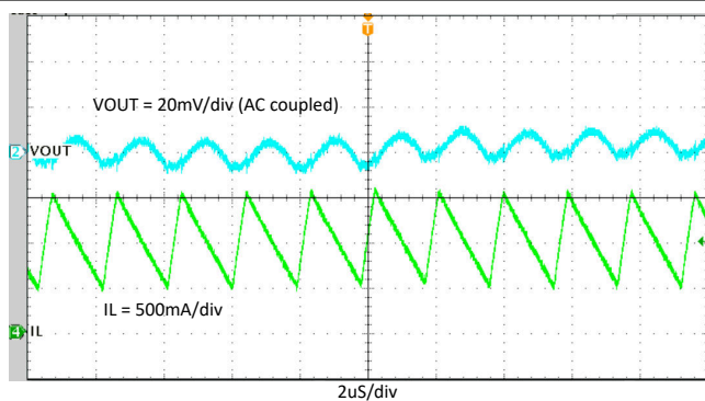
FIG 10-16. Steady State, I_{OUT} = 1 A
