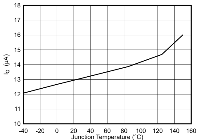
FIG 8-1. TPS62933 Quiescent Current vs Junction Temperature
