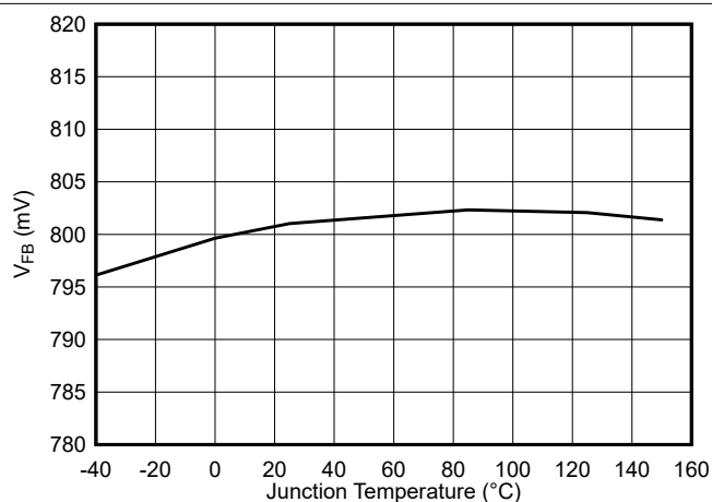
FIG 8-5. Feedback Voltage vs Junction Temperature
