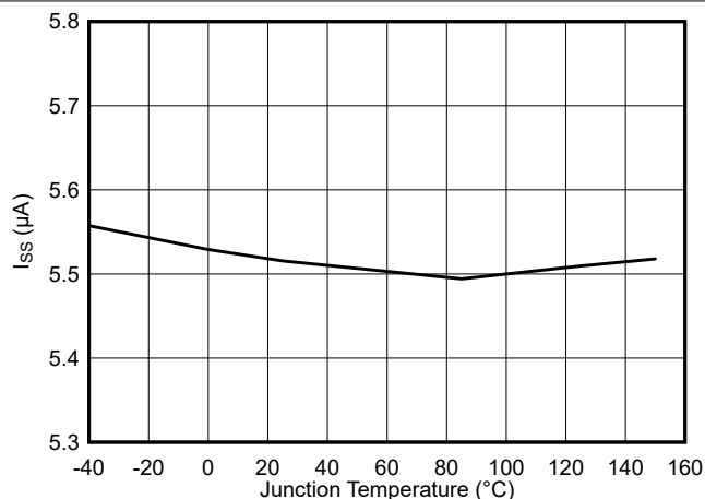
FIG 8-17. Soft-Start Charge Current vs Junction Temperature
