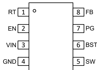
図 7-2. TPS62933P and TPS62933O 8-Pin SOT583 DRL Package (Top View)
