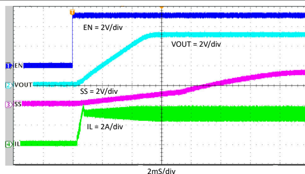
10-11. Start-Up Through EN, I_{OUT} = 3\text{ A}
