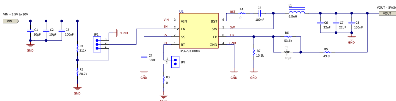
10-1. TPS62933 5-V Output, 3-A Reference Design
