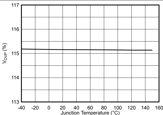
FIG 8-15. OVP Threshold vs Junction Temperature
