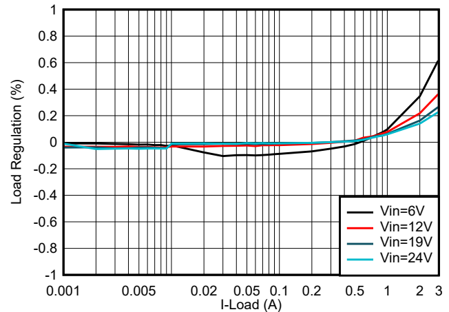
8-28. TPS62933F Load Regulation, V_{OUT} = 5\text{ V} , f_{SW} = 500\text{ kHz}
