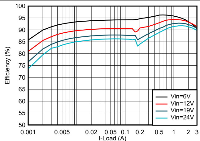
FIG 8-18. TPS62933 Efficiency, V_{OUT} = 3.3\text{ V} , f_{SW} = 500\text{ kHz} , L = 4.7\text{ }\mu\text{H}
