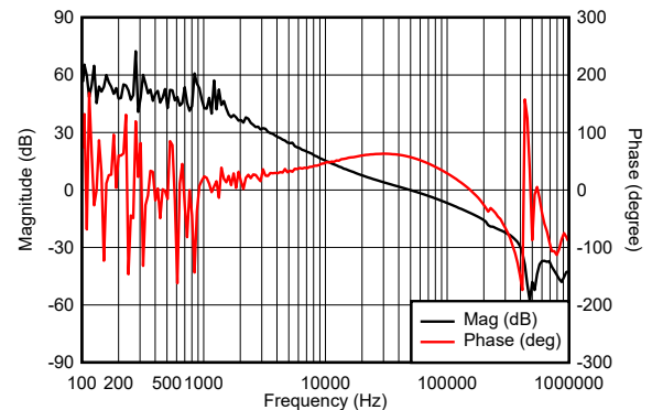
FIG 10-7. Loop Frequency Response, I_{OUT} = 3\text{ A} , BW = 49.4 kHz, PM = 57°, GM = -12 dB
