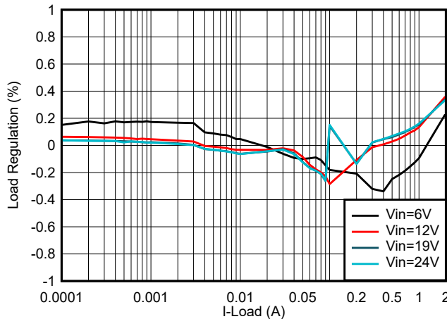
8-27. TPS62932 Load Regulation, V_{OUT} = 5\text{ V} , f_{SW} = 500\text{ kHz}
