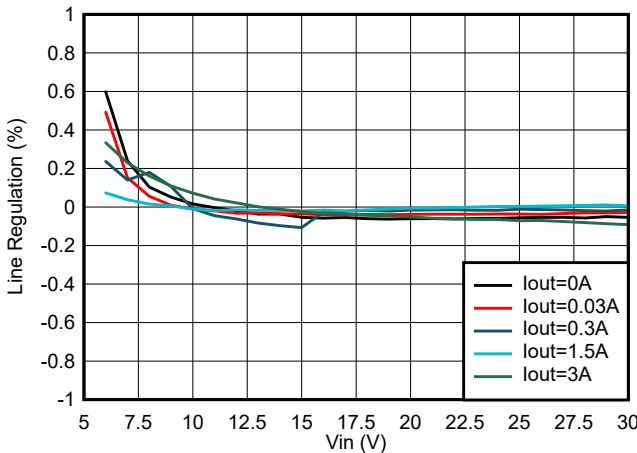
FIG 10-4. Line Regulation
