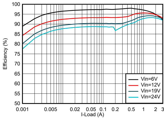
FIG 10-2. Efficiency
