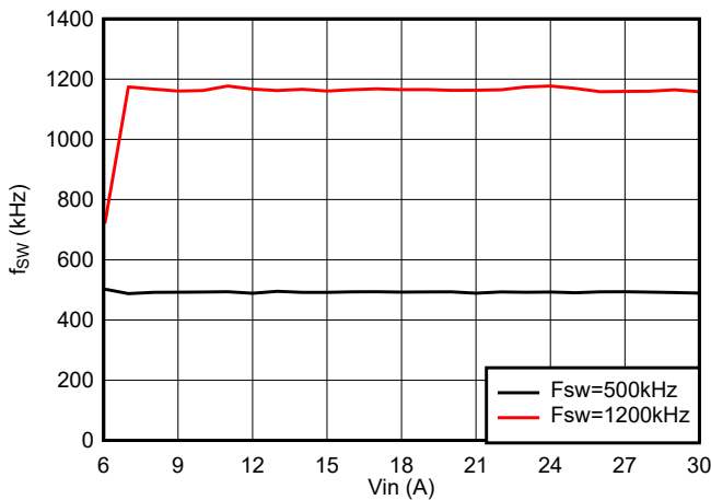
FIG 10-6. Switching Frequency vs V_{IN} , V_{OUT} = 5\text{ V}
