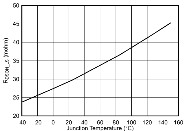
FIG 8-4. Low-Side R_{DS(on)} vs Junction Temperature
