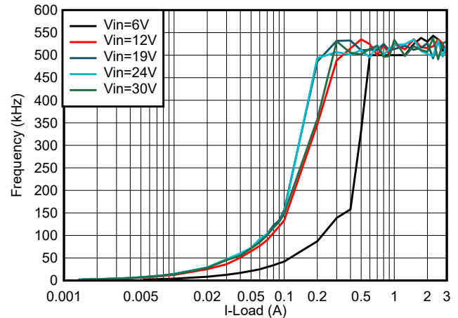
FIG 10-5. Switching Frequency vs Load Current
