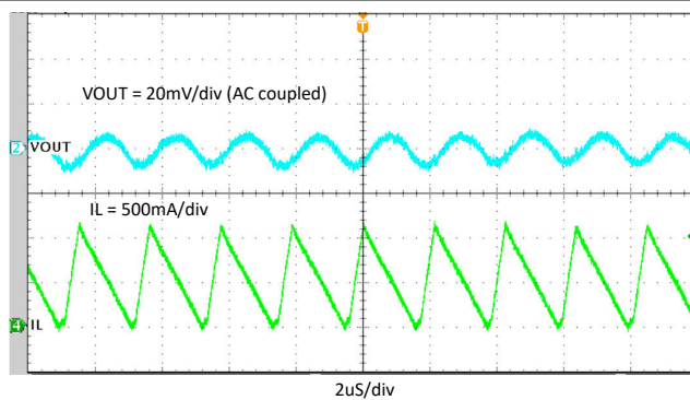
FIG 10-15. Steady State, I_{OUT} = 0.5 A
