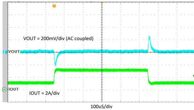
10-20. Load Transient Response, 1 to 3 A, Slew Rate = 0.8 A/μS
