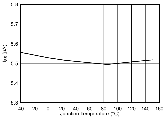
FIG 8-17. Soft-Start Charge Current vs Junction Temperature
