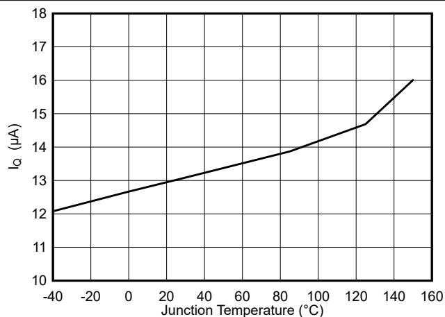
FIG 8-1. TPS62933 Quiescent Current vs Junction Temperature
