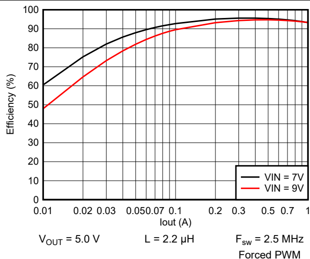
Figure 9-3. Efficiency vs Output Current
