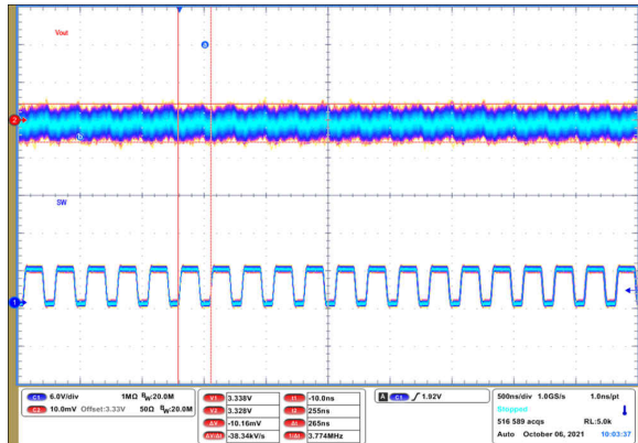
Figure 9-70. Output Voltage Ripple
