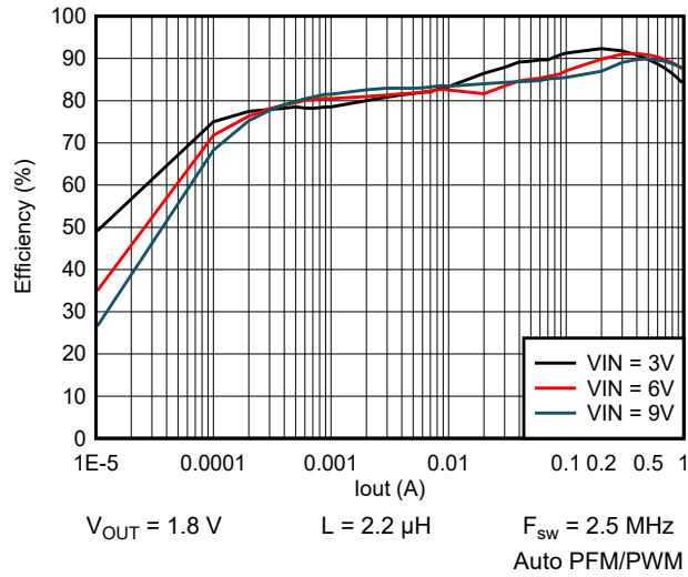
9-26. Efficiency vs Output Current
