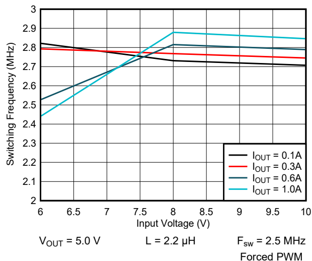
Figure 9-5. Switching Frequency vs Input Voltage
