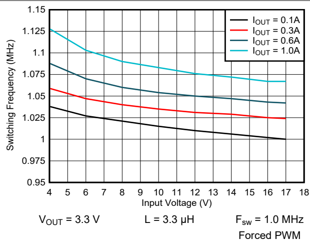
图 9-23. Switching Frequency vs Input Voltage
