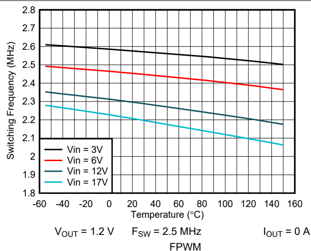
FIG 7-9. Switching Frequency vs Temperature
