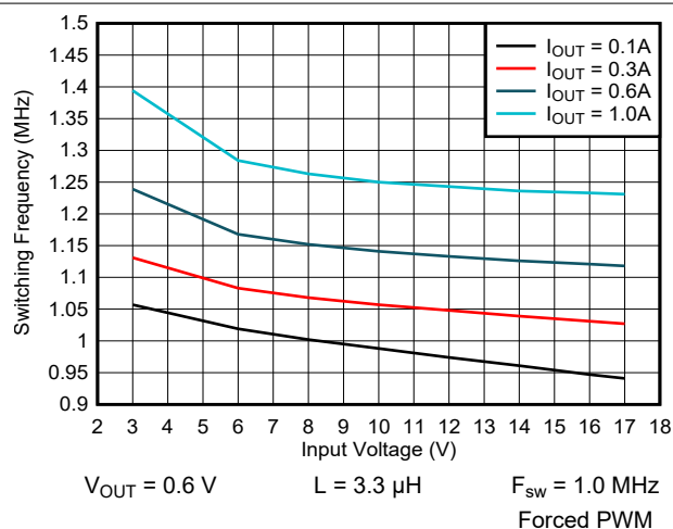
Figure 9-59. Switching Frequency vs Input Voltage
