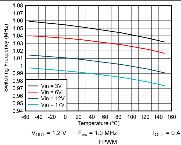
FIG 7-10. Switching Frequency vs Temperature
