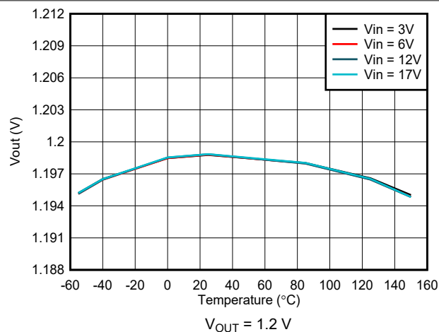
FIG 7-7. Output Voltage Accuracy – VSET Selected
