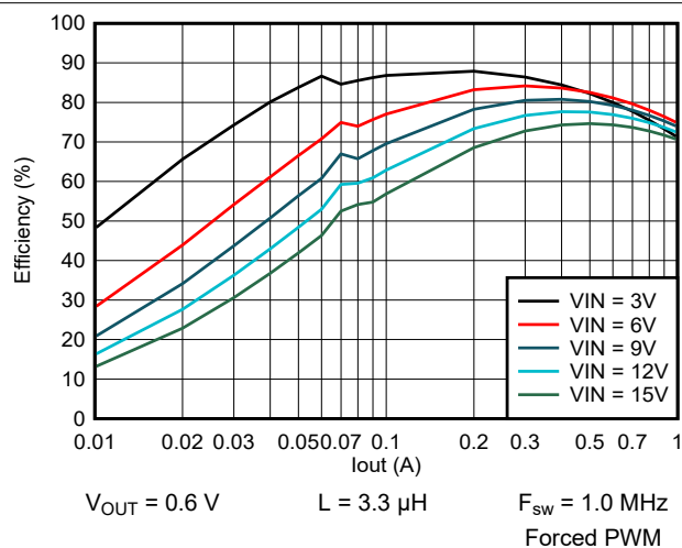
Figure 9-57. Efficiency vs Output Current
