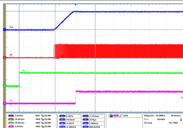
9-63. Start-Up Timing
