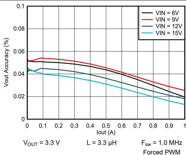
图 9-25. Output Voltage vs Output Current
