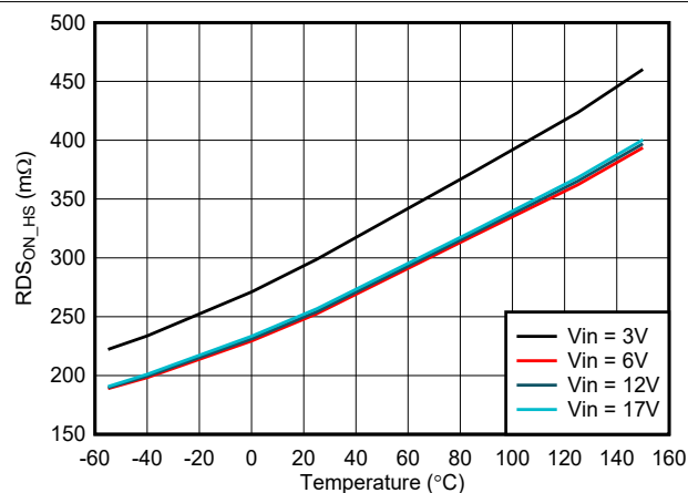
FIG 7-11. High-Side R_{DS(on)} vs Temperature
