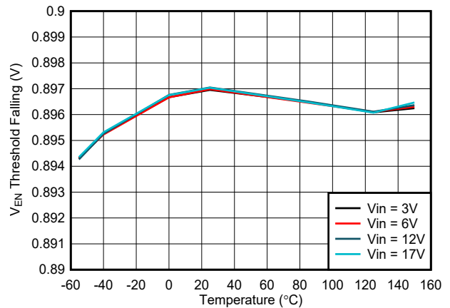
FIG 7-18. Precision Enable Threshold vs Temperature
