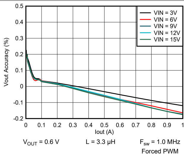
Figure 9-61. Output Voltage vs Output Current
