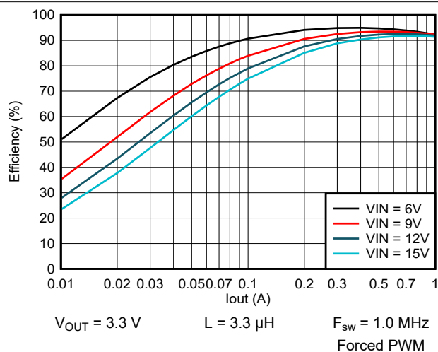
图 9-21. Efficiency vs Output Current
