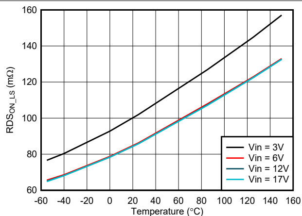
FIG 7-12. Low-Side R_{DS(on)} vs Temperature
