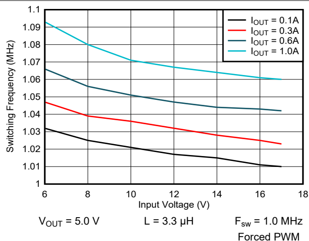
Figure 9-11. Switching Frequency vs Input Voltage
