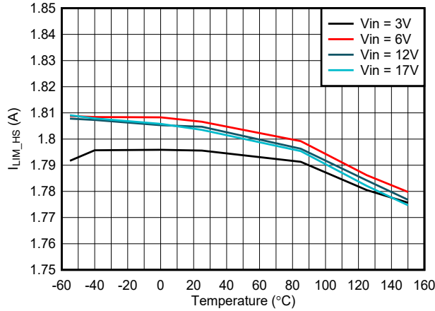
FIG 7-13. High-Side I_{LIM} vs Temperature
