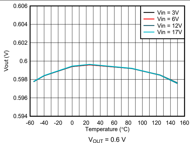
FIG 7-8. Output Voltage Accuracy – VSET Selected
