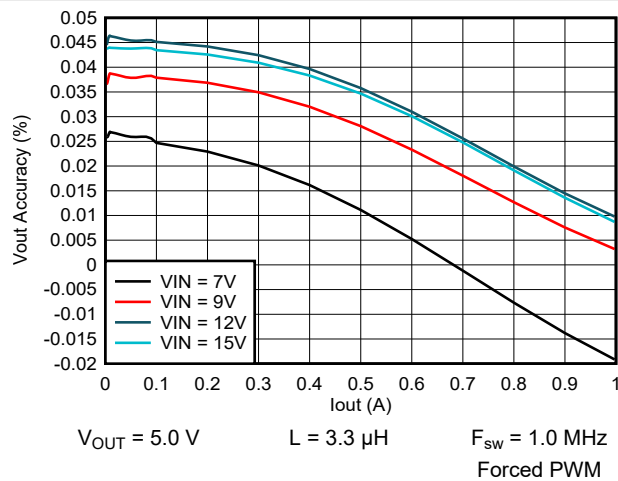
Figure 9-13. Output Voltage vs Output Current
