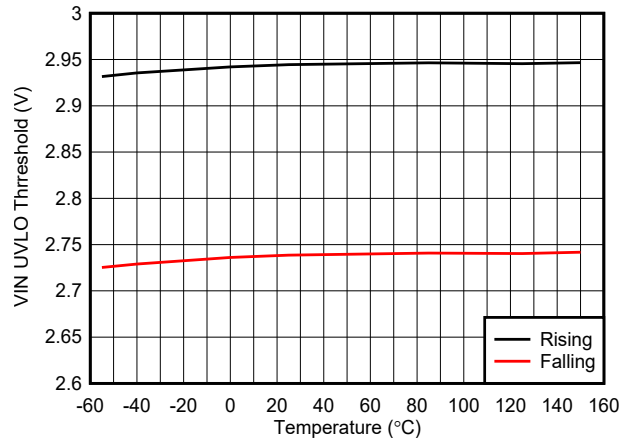
FIG 7-16. V_{IN} UVLO Thresholds vs Temperature
