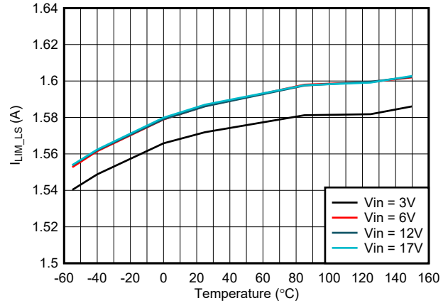
FIG 7-14. Low-Side I_{LIM} vs Temperature
