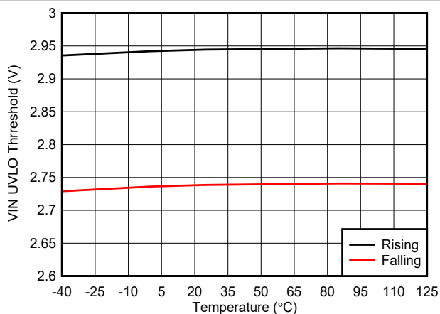
FIG 7-16. V_{IN} UVLO Thresholds vs Temperature
