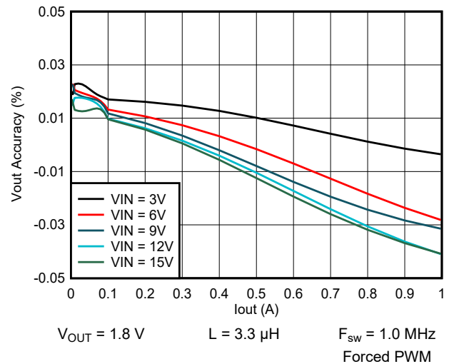
9-37. Output Voltage vs Output Current
