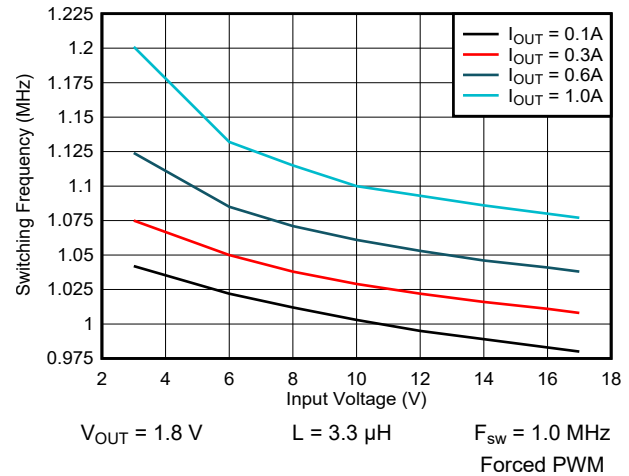
9-35. Switching Frequency vs Input Voltage
