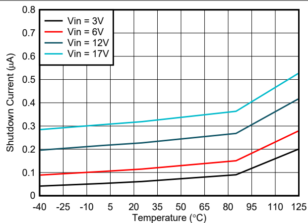
7-2. Typical Shutdown Current vs Temperature
