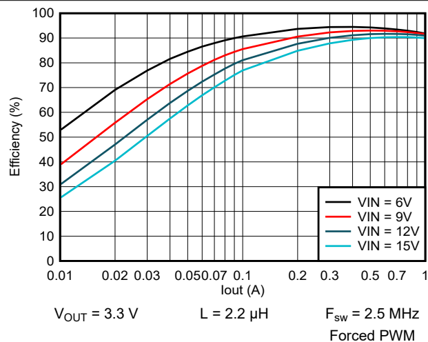
9-15. Efficiency vs Output Current
