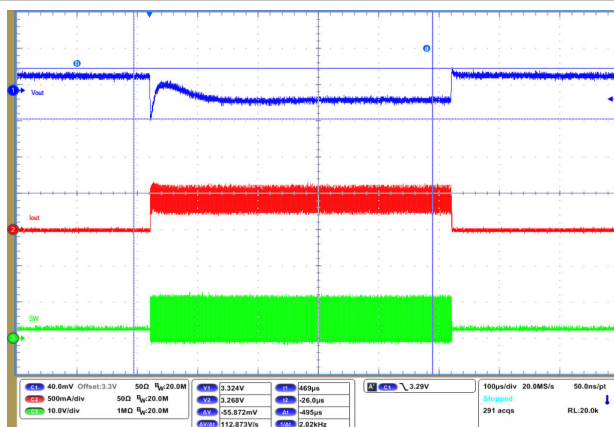
FIG 9-69. Shutdown Timing with Output Discharge Enabled
