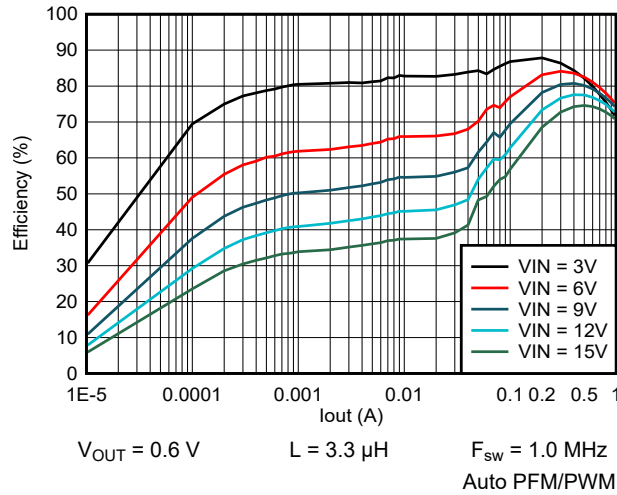
9-56. Efficiency vs Output Current
