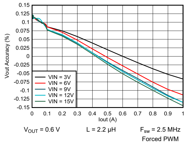
9-55. Output Voltage vs Output Current
