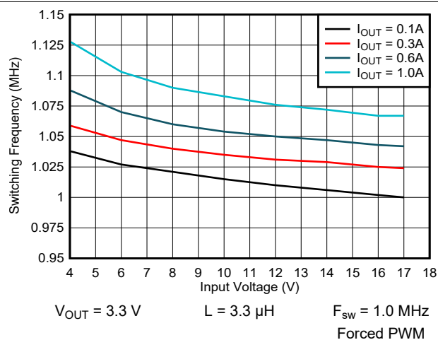
9-23. Switching Frequency vs Input Voltage
