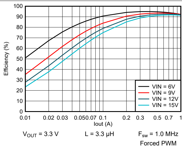
9-21. Efficiency vs Output Current
