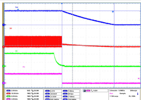
FIG 9-68. Shutdown Timing with Output Discharge Disabled
