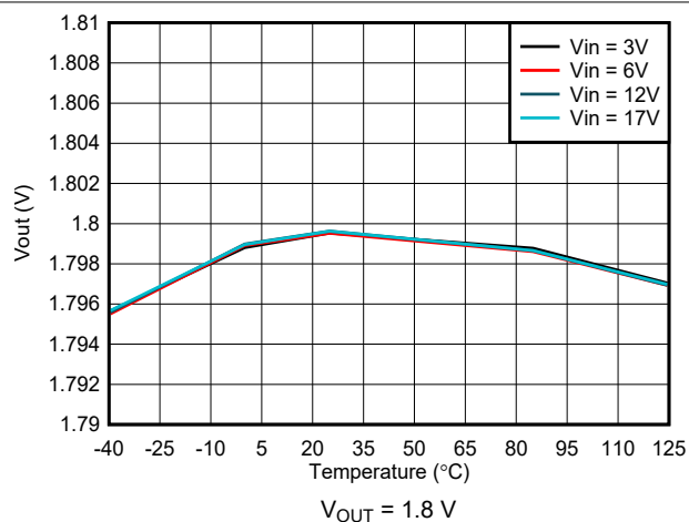
7-6. Output Voltage Accuracy – VSET Selected
