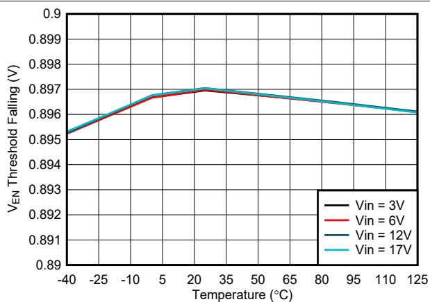
FIG 7-18. Precision Enable Threshold vs Temperature
