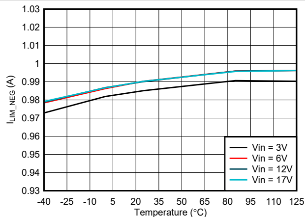
FIG 7-15. Low-Side I_{NEG} vs Temperature
