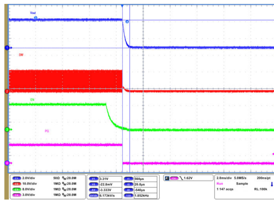
FIG 9-69. Shutdown Timing with Output Discharge Enabled
