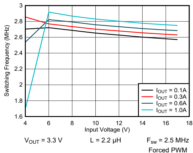
9-17. Switching Frequency vs Input Voltage
