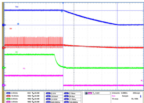
FIG 9-68. Shutdown Timing with Output Discharge Disabled
