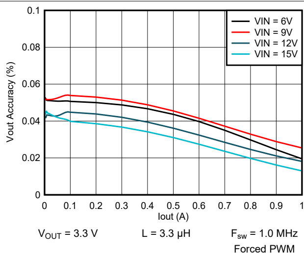
9-25. Output Voltage vs Output Current
