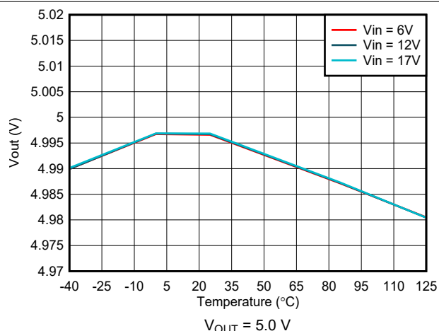
7-4. Output Voltage Accuracy – VSET Selected
