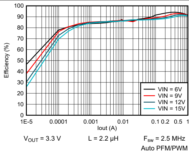
9-14. Efficiency vs Output Current
