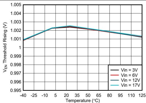
FIG 7-17. Precision Enable Threshold vs Temperature
