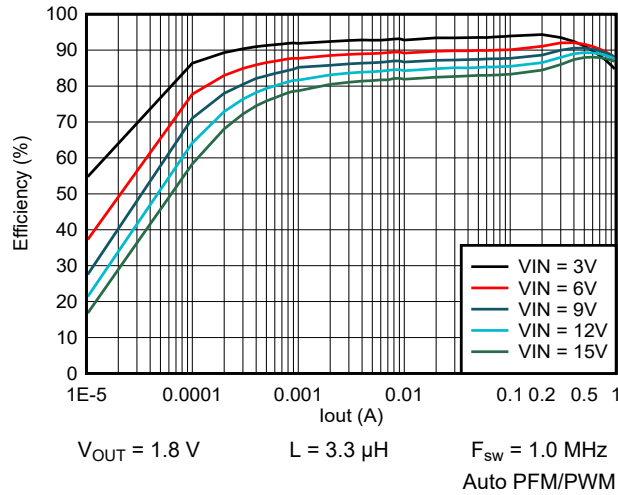
9-32. Efficiency vs Output Current
