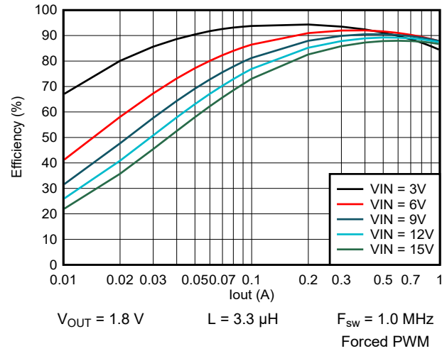
9-33. Efficiency vs Output Current
