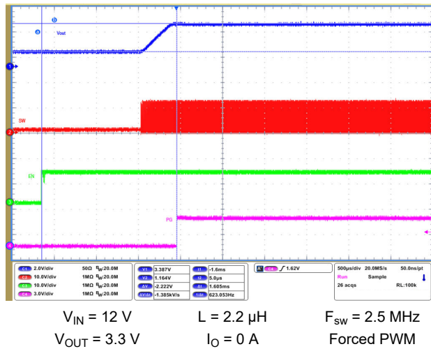
9-64. Start-Up into Prebiased Output
