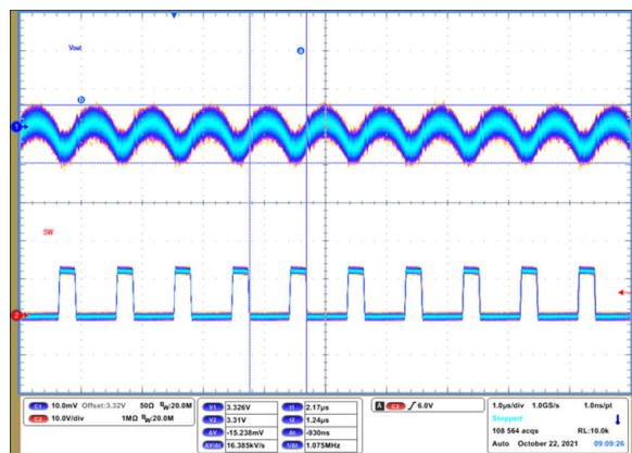
9-74. Output Voltage Ripple
