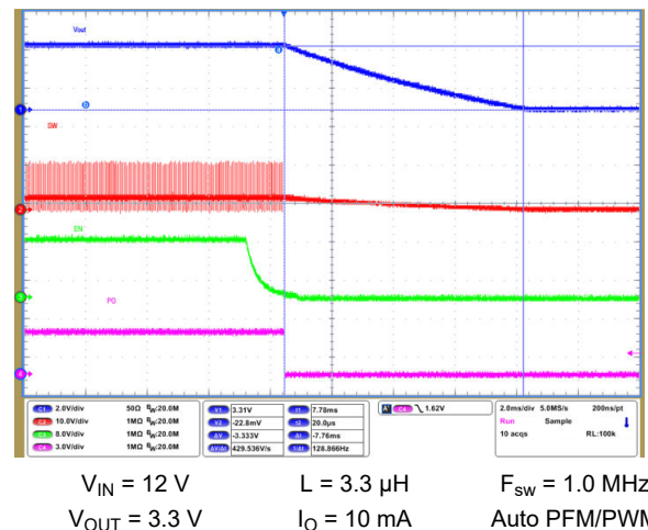
9-67. Shutdown Timing with Output Discharge Disabled
