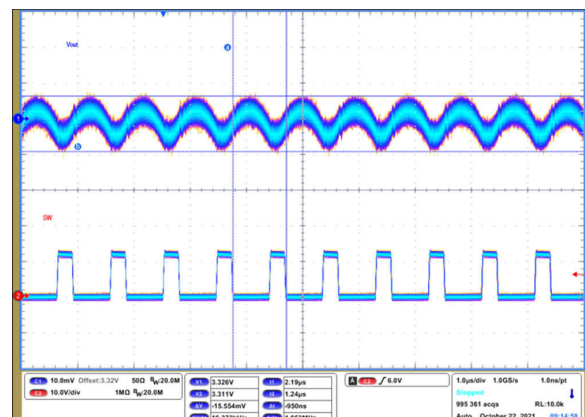
9-75. Output Voltage Ripple
