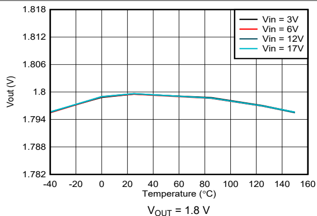
Figure 7-6. Output Voltage Accuracy – VSET Selected
