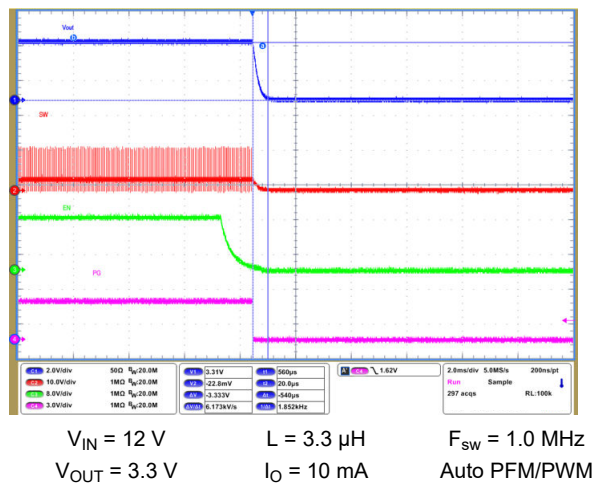
9-66. Shutdown Timing with Output Discharge Enabled
