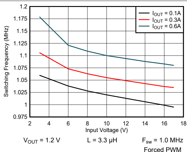
9-47. Switching Frequency vs Input Voltage
