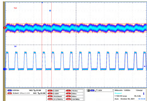
9-75. Output Voltage Ripple
