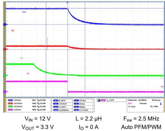
9-65. Shutdown Timing with Output Discharge Enabled
