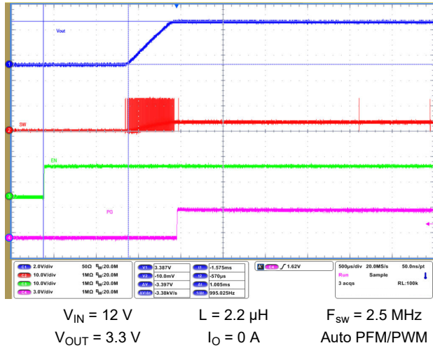
9-62. Start-Up Timing
