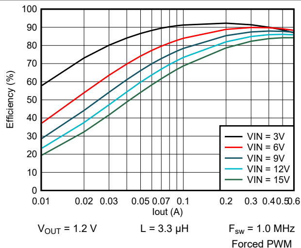
9-45. Efficiency vs Output Current
