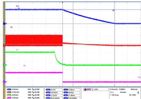
FIG 9-69. Shutdown Timing with Output Discharge Disabled
