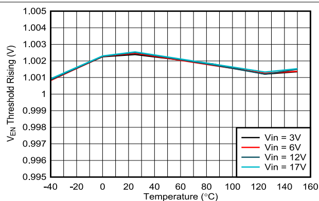
7-17. Precision Enable Threshold vs Temperature
