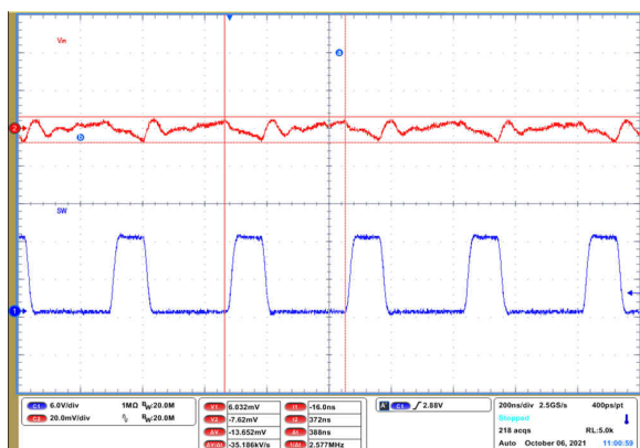
9-76. Output Voltage Ripple
