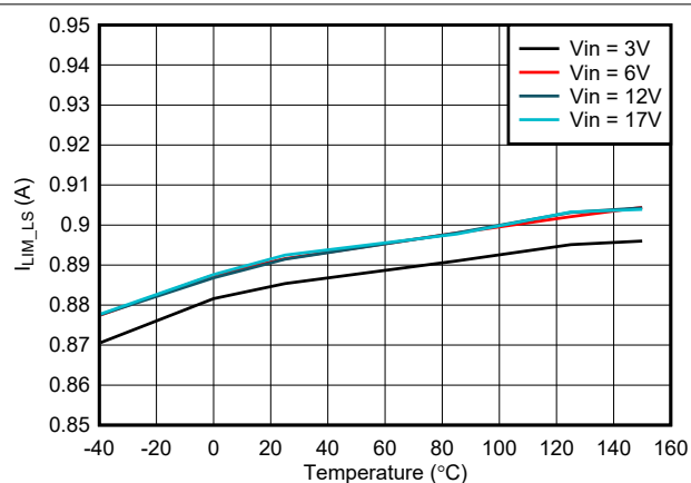
7-14. Low-Side I_{LIM} vs Temperature
