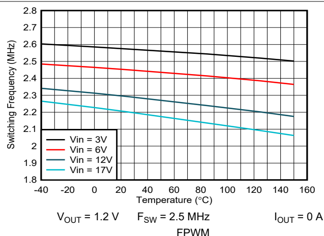
7-9. Switching Frequency vs Temperature
