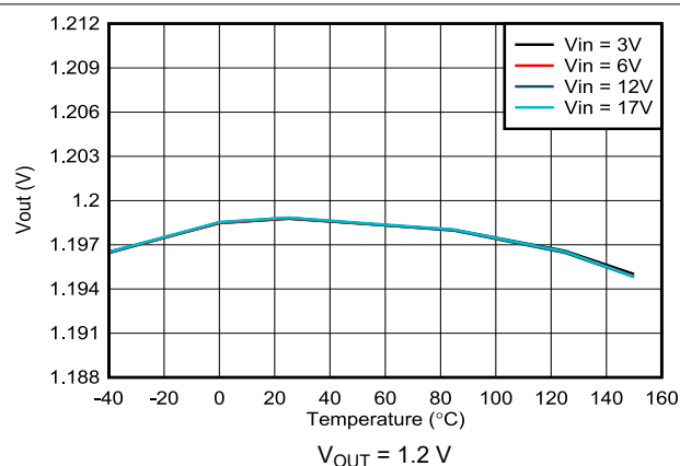
7-7. Output Voltage Accuracy – VSET Selected
