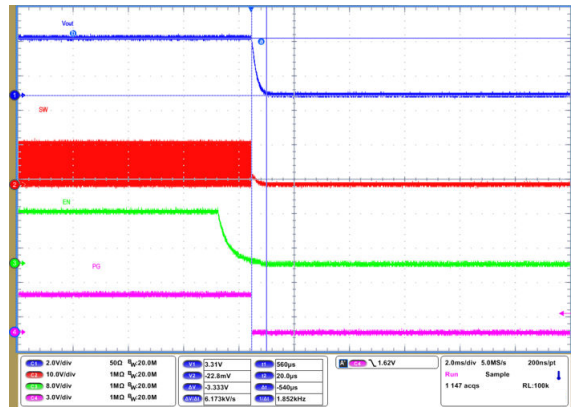
FIG 9-68. Shutdown Timing with Output Discharge Enabled
