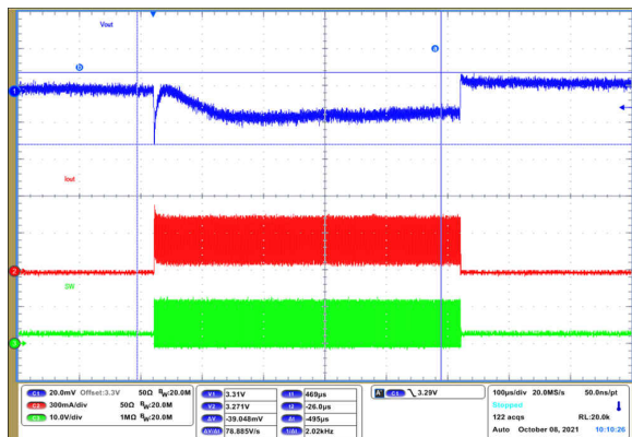
FIG 9-68. Shutdown Timing with Output Discharge Enabled
