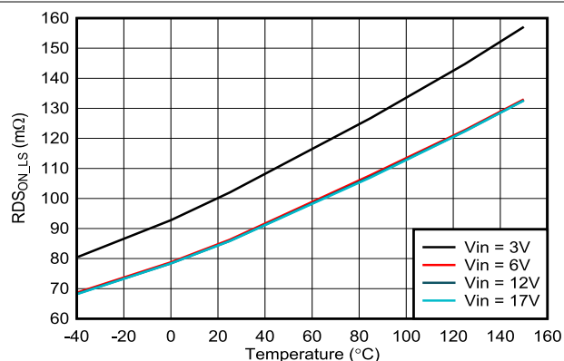
7-12. Low-Side R_{DS(on)} vs Temperature
