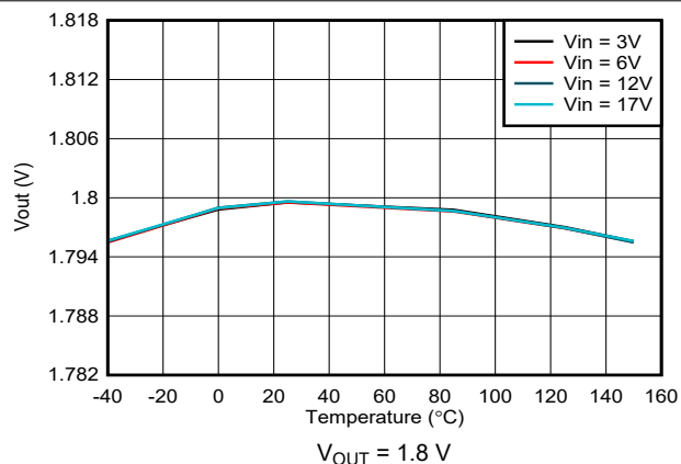
FIG 7-6. Output Voltage Accuracy – VSET Selected
