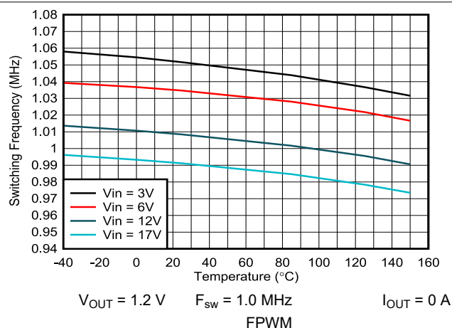
7-10. Switching Frequency vs Temperature
