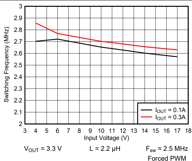
9-17. Switching Frequency vs Input Voltage
