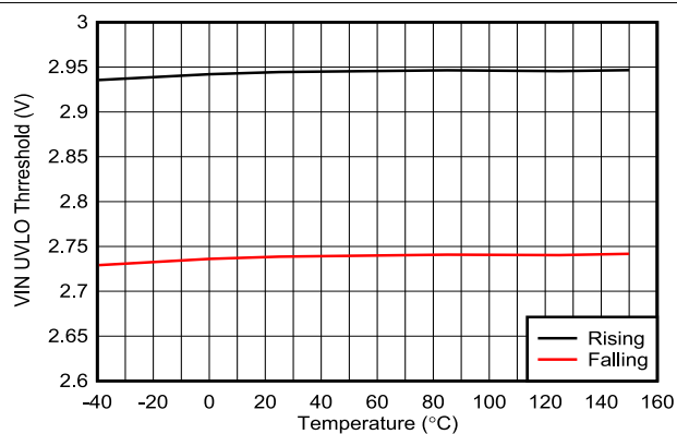
7-16. V_{IN} UVLO Thresholds vs Temperature
