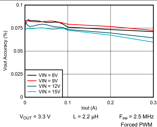
9-19. Output Voltage vs Output Current
