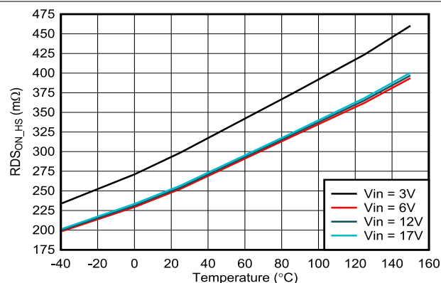
7-11. High-Side R_{DS(on)} vs Temperature
