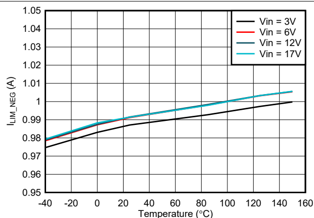
7-15. Low-Side I_{NEG} vs Temperature
