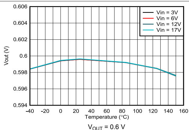
7-8. Output Voltage Accuracy – VSET Selected
