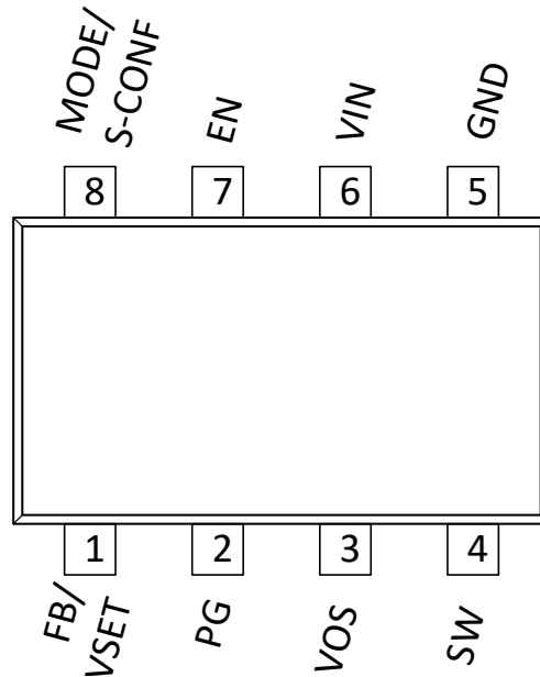
図 6-1. TPS629203-Q1 8-Pin DRL SOT-5X3 Pinout
