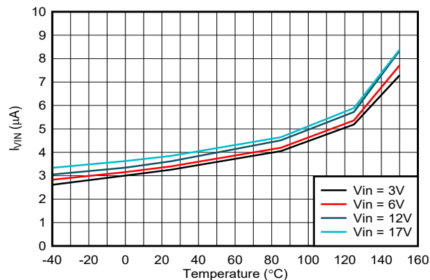
FIG 7-1. Typical Quiescent Current vs Temperature
