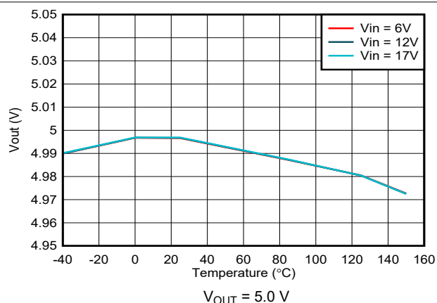
FIG 7-4. Output Voltage Accuracy – VSET Selected
