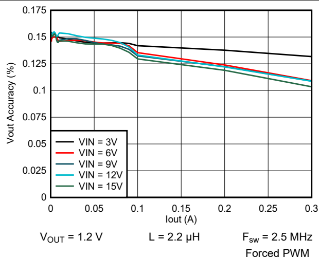
9-43. Output Voltage vs Output Current
