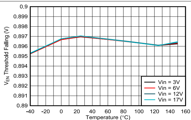
7-18. Precision Enable Threshold vs Temperature
