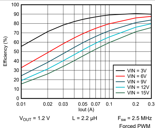
9-39. Efficiency vs Output Current
