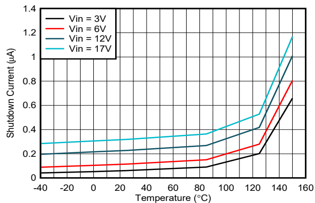
FIG 7-2. Typical Shutdown Current vs Temperature
