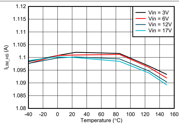
7-13. High-Side I_{LIM} vs Temperature
