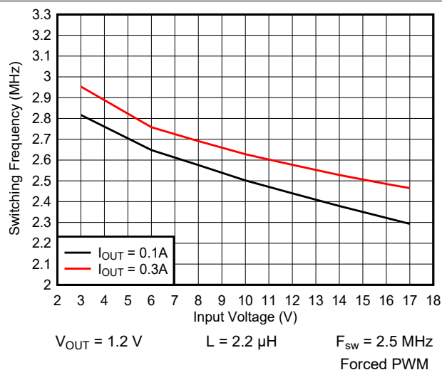
9-41. Switching Frequency vs Input Voltage
