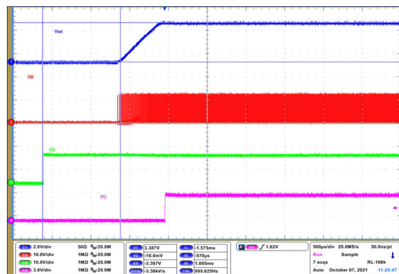
Figure 9-63. Start-Up Timing
