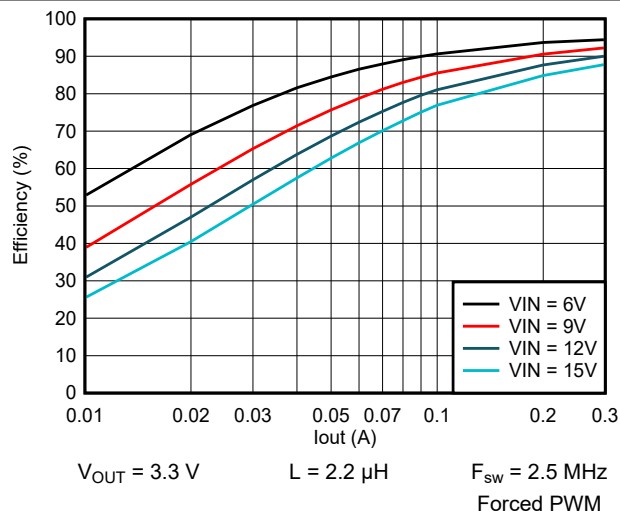
9-15. Efficiency vs Output Current
