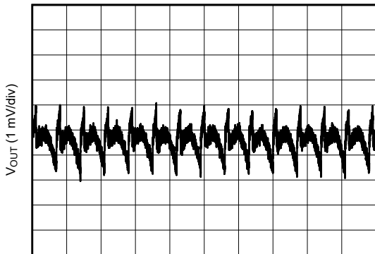
図 5-3. V_{OUT} Ripple After the Second L-C Filter
