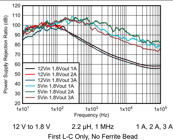
Figure 6-47. PSRR vs Frequency
