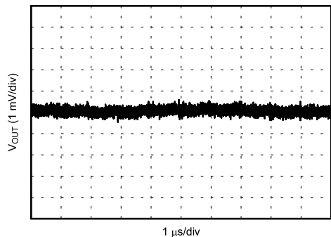
FIG 6-7. V_{OUT} Ripple After the First L-C Filter
