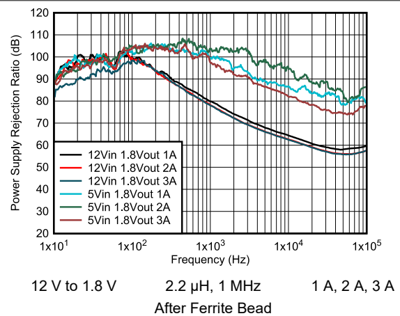
Figure 6-48. PSRR vs Frequency
