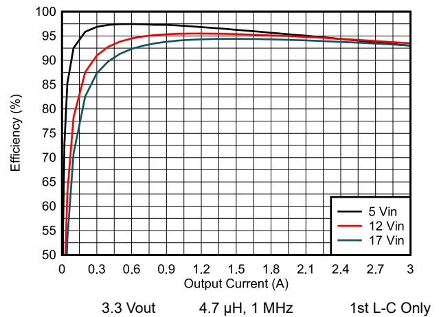
8-5. Efficiency vs Load Current
