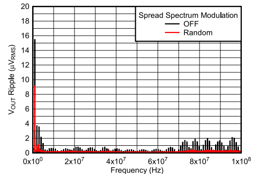
FIG 6-8. V_{OUT} Ripple FFT After the First L-C Filter
