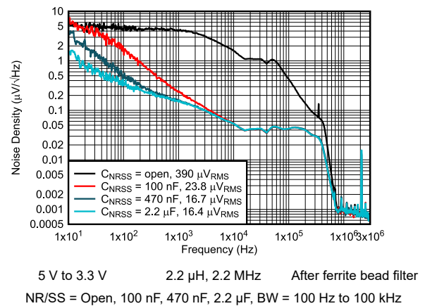
Figure 6-44. Output Noise Density vs Frequency
