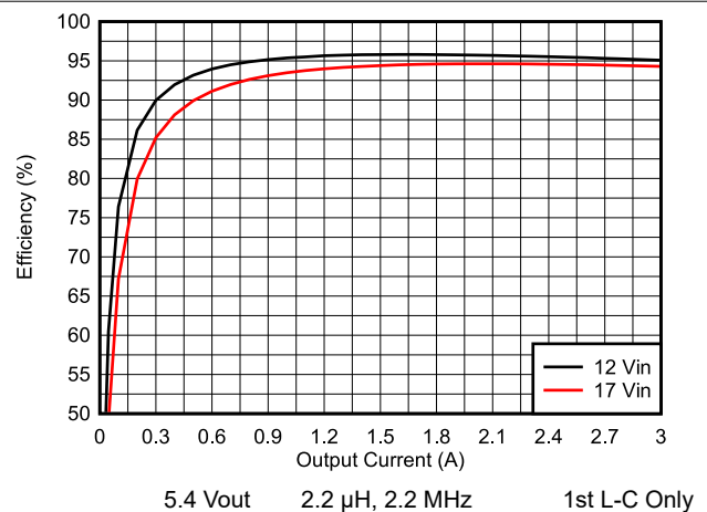
8-7. Efficiency vs Load Current
