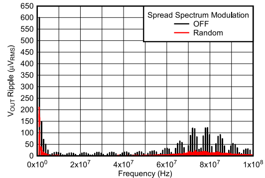
FIG 6-8. V_{OUT} Ripple FFT After the First L-C Filter
