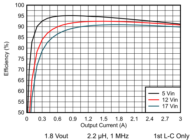
8-4. Efficiency vs Load Current
