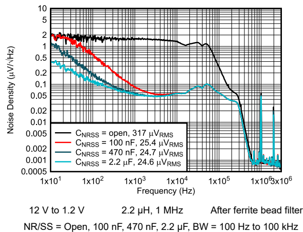
Figure 6-30. Output Noise Density vs Frequency
