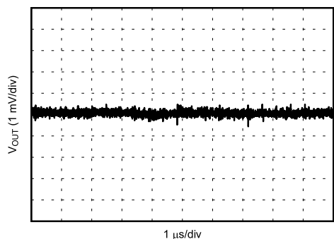
Figure 6-25. V_{OUT} Ripple After the Second L-C Filter
