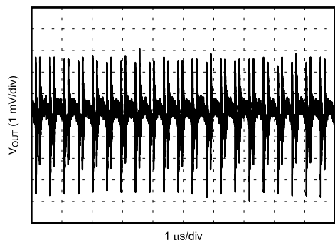
FIG 6-9. V_{OUT} Ripple After the Second L-C Filter
