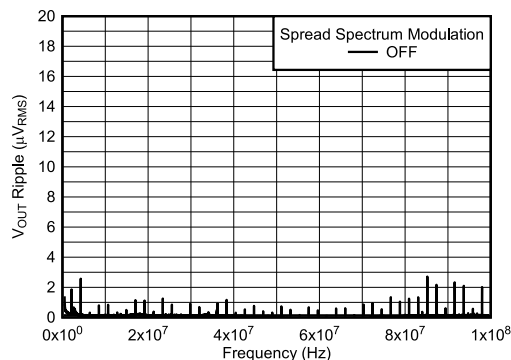
Figure 6-26. V_{OUT} Ripple FFT After the Second L-C Filter
