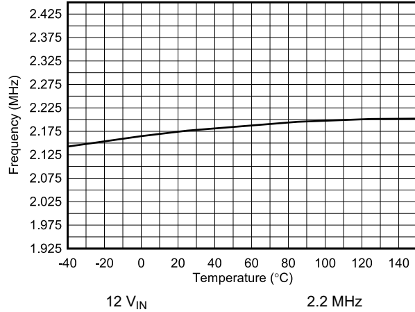
6-55. Oscillator Frequency vs Temperature
