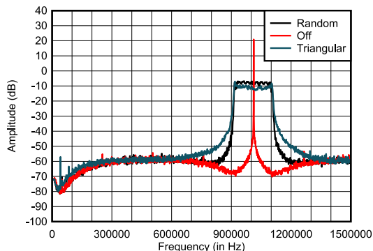
Figure 6-25. V_{OUT} Ripple After the Second L-C Filter
