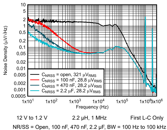
Figure 6-29. Output Noise Density vs Frequency
