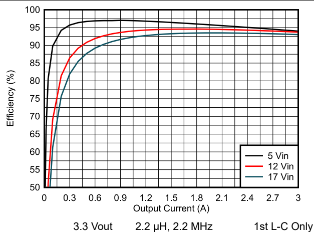
8-6. Efficiency vs Load Current
