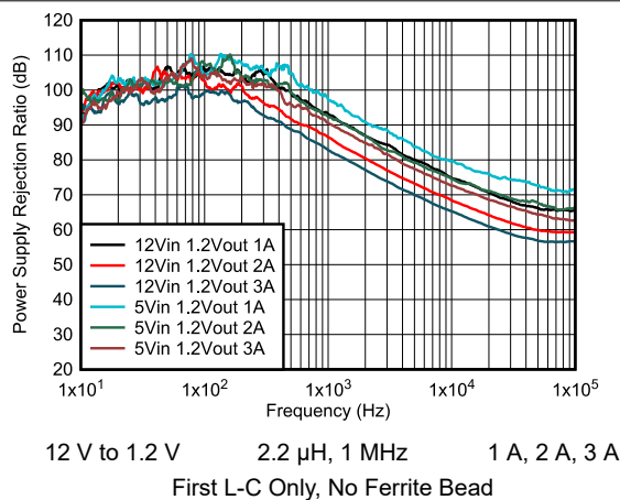
Figure 6-45. PSRR vs Frequency
