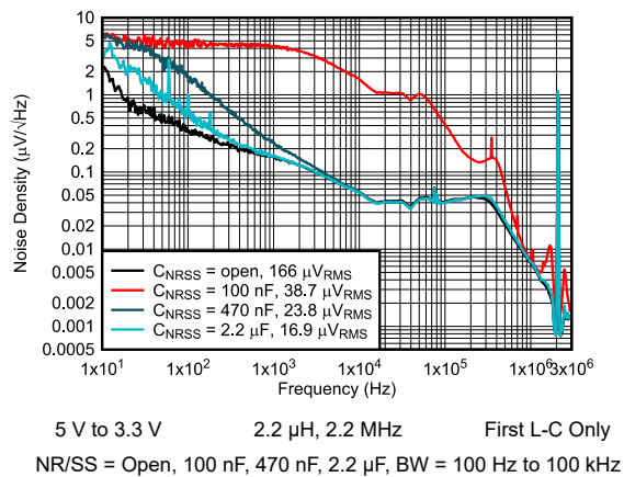
Figure 6-43. Output Noise Density vs Frequency
