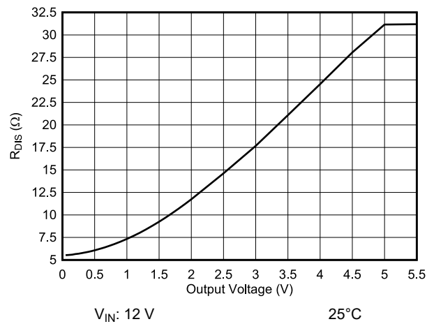
6-57. Output Discharge Resistance vs Output Voltage
