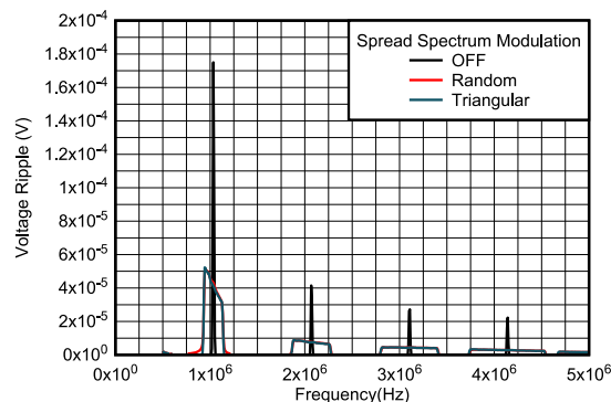
Figure 6-26. V_{OUT} Ripple FFT After the Second L-C Filter
