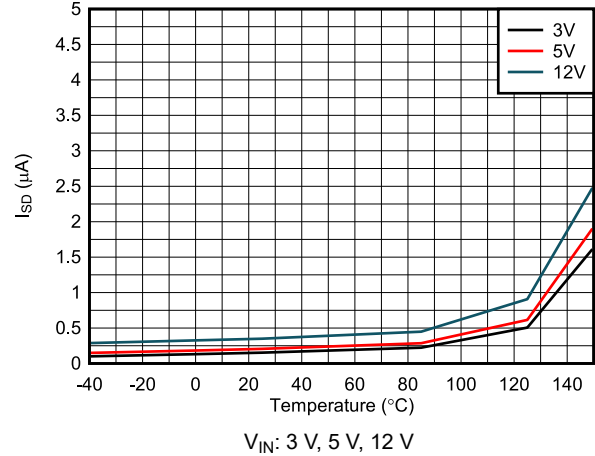
6-56. Shutdown Current vs Temperature
