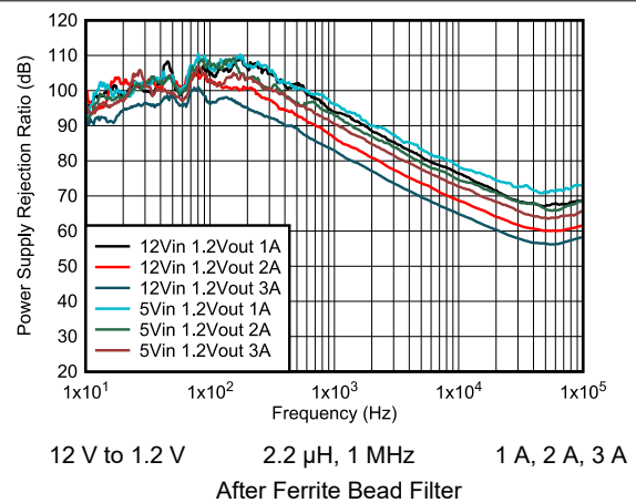
Figure 6-46. PSRR vs Frequency
