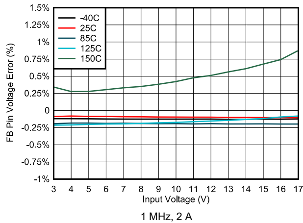
FIG 6-51. FB Pin Voltage Error vs Input Voltage
