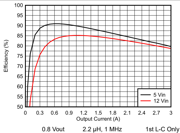
8-2. Efficiency vs Load Current
