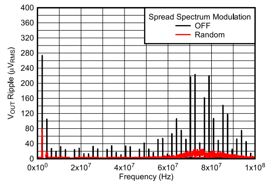
FIG 6-10. V_{OUT} Ripple FFT After the Second L-C Filter
