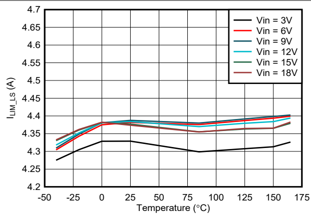
FIG 7-16. Low Side I_{LIM} vs Temperature
