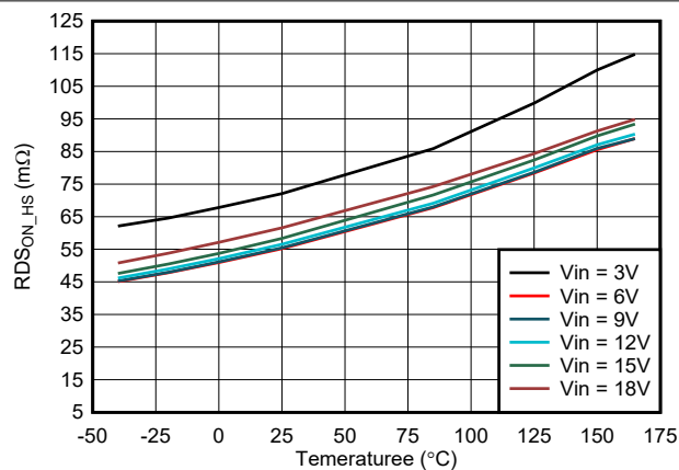
FIG 7-13. High Side R_{DS(ON)} vs Temperature
