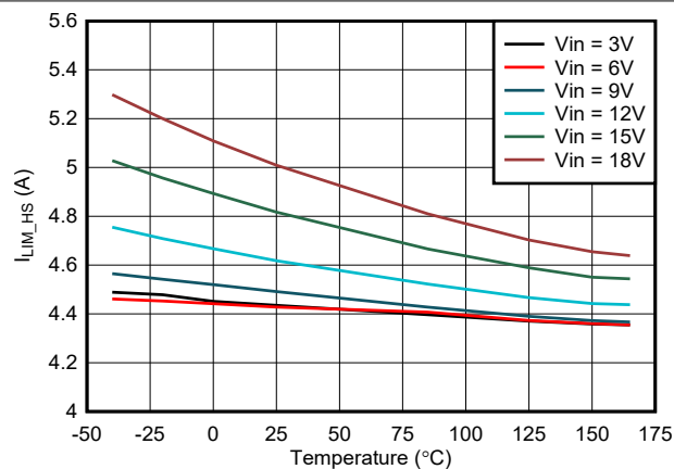
FIG 7-15. High Side I_{LIM} vs Temperature
