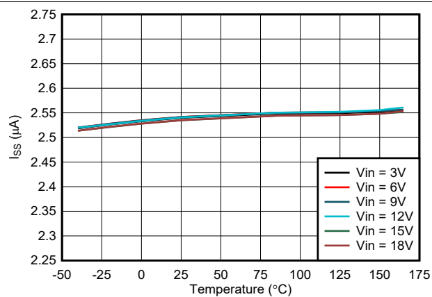
FIG 7-18. Soft Start Current vs Temperature
