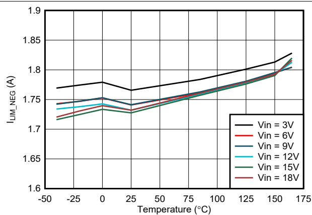
FIG 7-17. Negative I_{LIM} vs Temperature
