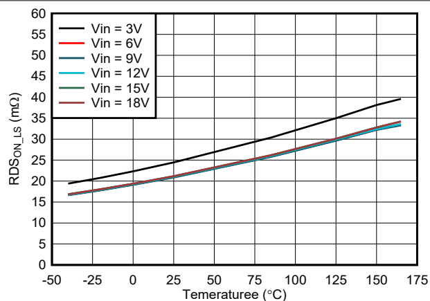
FIG 7-14. Low Side R_{DS(ON)} vs Temperature
