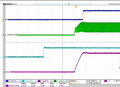
V_{IN} = 12\text{ V} 1 MHz Auto I_O = 1\text{ A} PFM/PWM V_{OUT} = 5\text{ V} T_A = 25^\circ\text{C}
