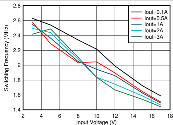
FPWM L = 1 \mu\text{H} F_{\text{sw}} = 2.5 \text{ MHz}
