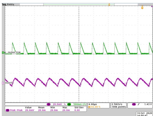
V_{IN} = 12\text{ V} 2.5 MHz Auto I_O = 0.1\text{ A} PFM/PWM V_{OUT} = 1.2\text{ V} L = 2.2\text{ }\mu\text{H} T_A = 25^\circ\text{C}
