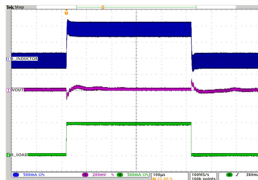
Figure 8-54. Typical Operation
