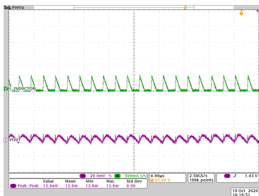
V_{IN} = 12\text{ V} 1 MHz Auto I_O = 0.1\text{ A} PFM/PWM V_{OUT} = 1.2\text{ V} L = 2.2\text{ }\mu\text{H} T_A = 25^\circ\text{C}
