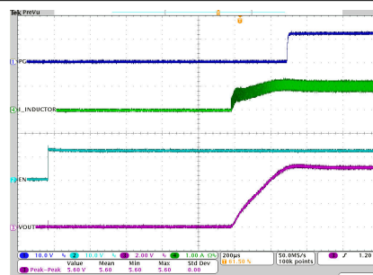
V_{IN} = 12\text{ V} 2.5 MHz Auto I_O = 1\text{ A} PFM/PWM V_{OUT} = 5\text{ V} T_A = 25^\circ\text{C}
