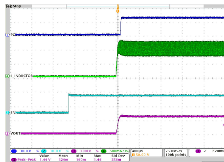
V_{\text{IN}} = 12 \text{ V} 1 \text{ MHz Auto PFM/PWM} I_{\text{O}} = 1 \text{ A} V_{\text{OUT}} = 1.2 \text{ V} T_{\text{A}} = 25^{\circ}\text{C}
