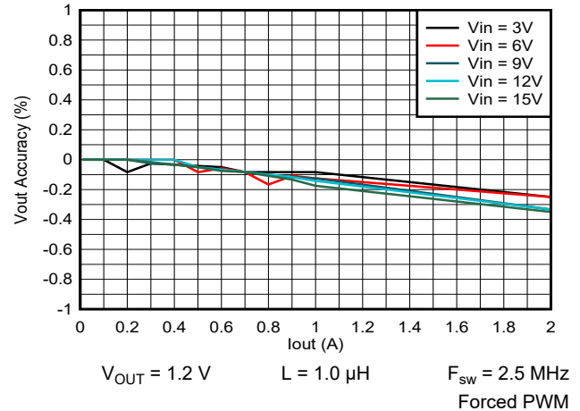
图 9-20. Output Voltage vs Output Current
