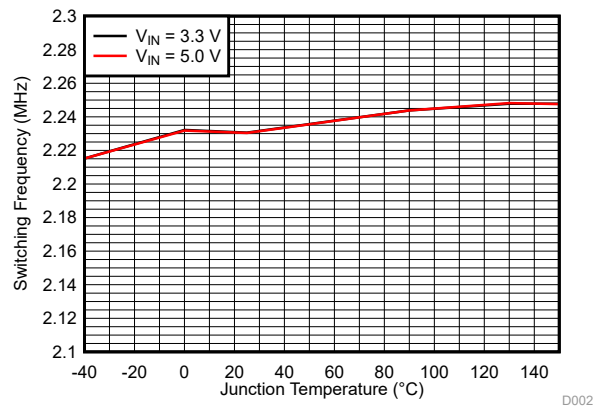
図 6-6. Switching Frequency vs Temperature
