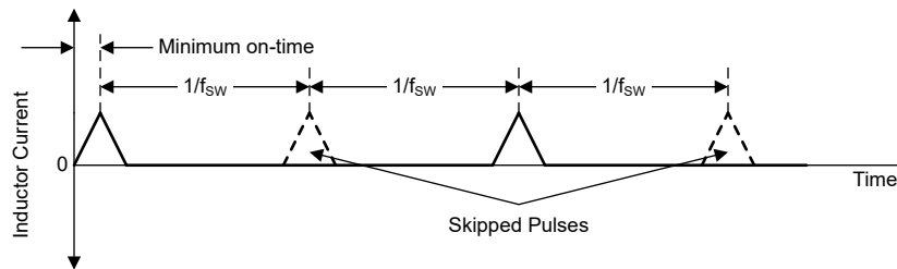
FIG 8-4. Discontinuous Conduction Mode (PFM-DCM) Current Waveform
