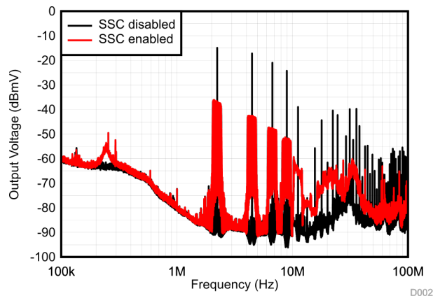
☒ 10-19. Output Voltage Noise
