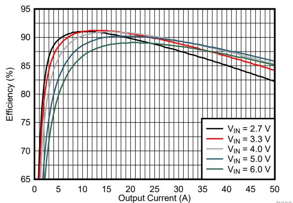
10-21. Efficiency Versus Output Current
