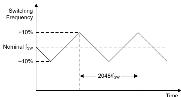
8-12. Spread Spectrum Clocking Behavior
