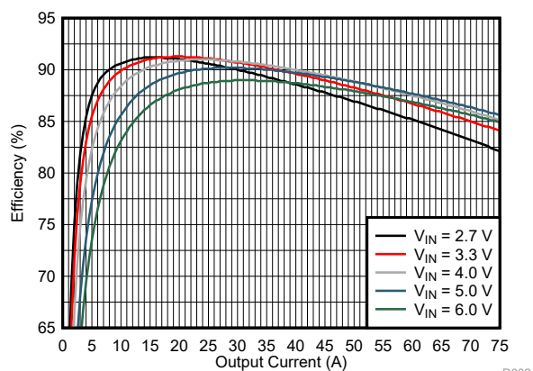
10-29. Efficiency Versus Output Current
