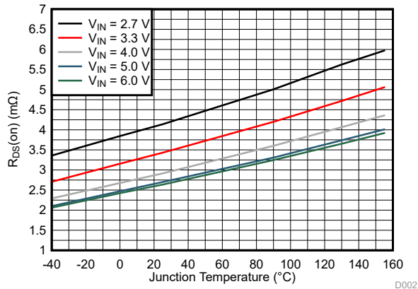
図 6-1. R_{DS(ON)} of High Side Switch
