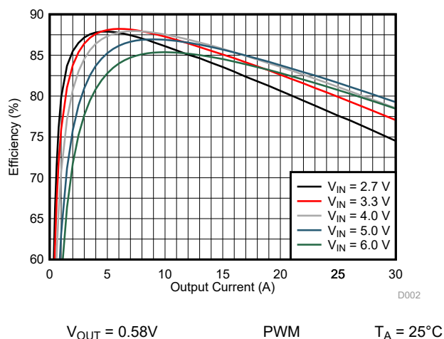
10-2. Efficiency Versus Output Current
