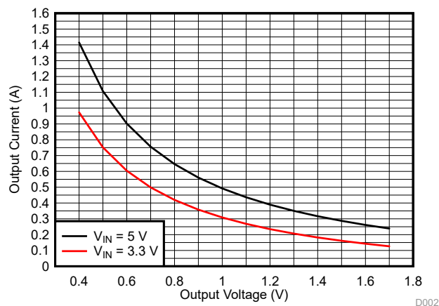
FIG 8-5. Output Current PFM-DCM Entry Threshold for f_{sw} = 2.25\text{MHz}
