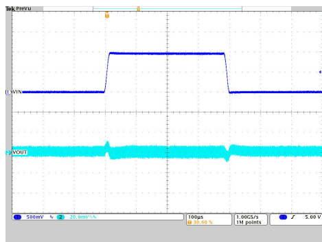
10-35. Line Transient Response
