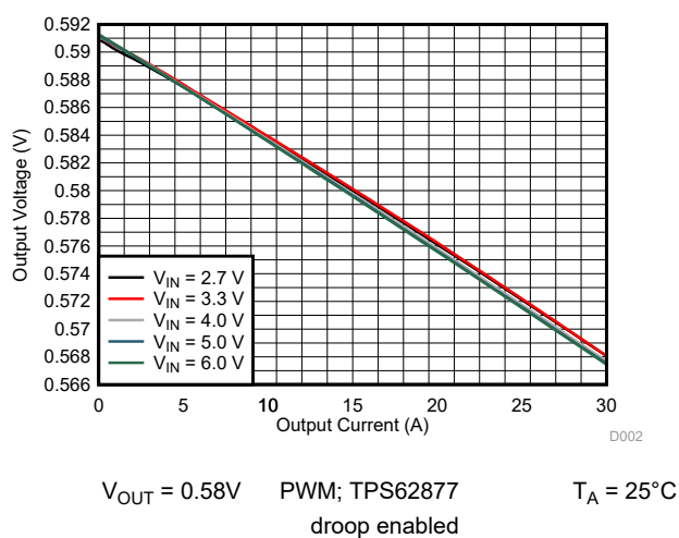
10-4. Output Voltage Versus Output Current
