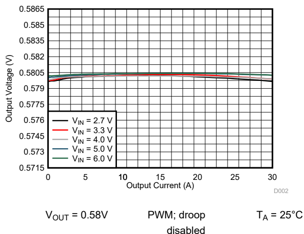
10-3. Output Voltage Versus Output Current
