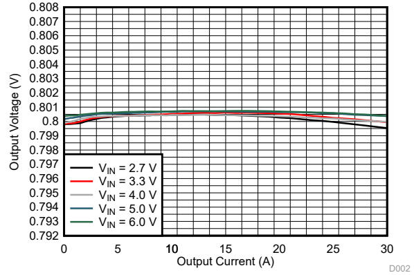
10-7. Output Voltage Versus Output Current
