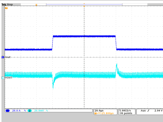
V_{OUT} = 0.8V T_A = 25^{\circ}C PWM; TPS62876 droop disabled V_{IN} = 5V I_{out} = 15A to 40A to 15A
