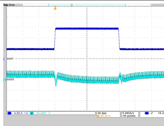
V_{OUT} = 0.75V PWM, TPS62874 droop enabled T_A = 25^\circ C V_{IN} = 5V I_{out} = 3.8A to 11.3A to 3.8A
