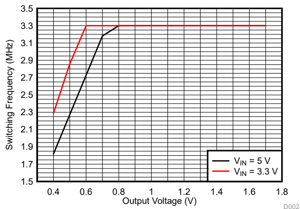
図 6-5. Maximum Switching Frequency vs Output Voltage
