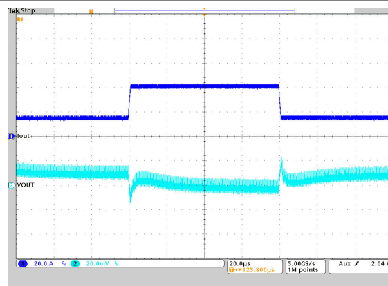
V_{OUT} = 0.8V T_A = 25^{\circ}C PWM; TPS62876 droop enabled V_{IN} = 5V I_{out} = 15A to 40A to 15A
