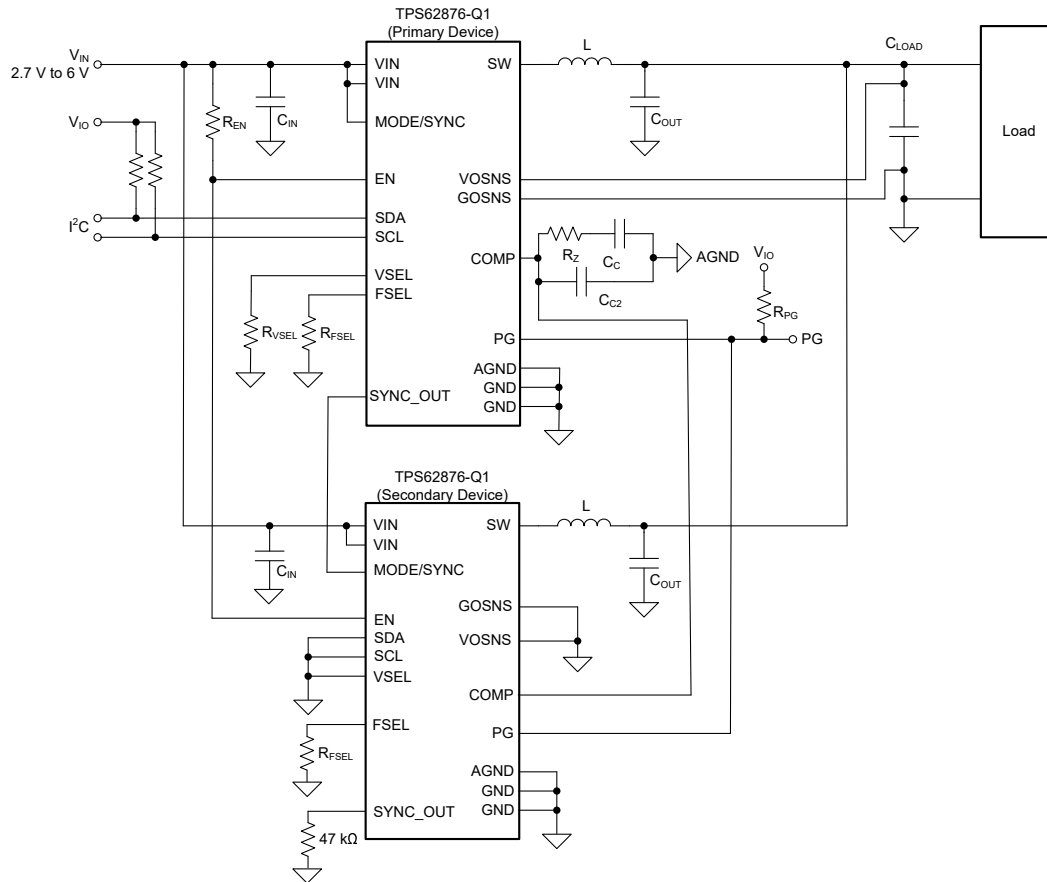
图 10-20. Stacking Two Devices
