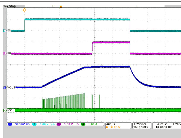
9-17. PSM Operation
