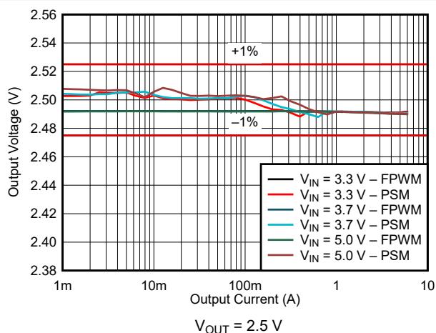
Figure 9-11. Load Regulation
