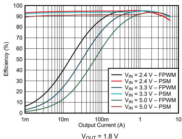
Figure 9-8. Efficiency
