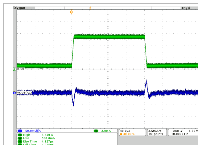
9-20. Load Transient - PWM Operation
