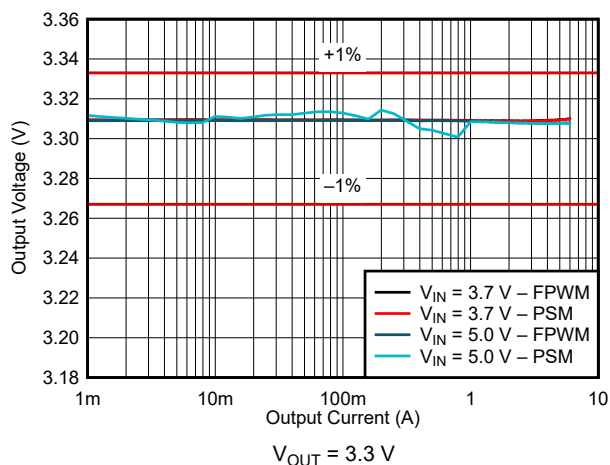
Figure 9-13. Load Regulation
