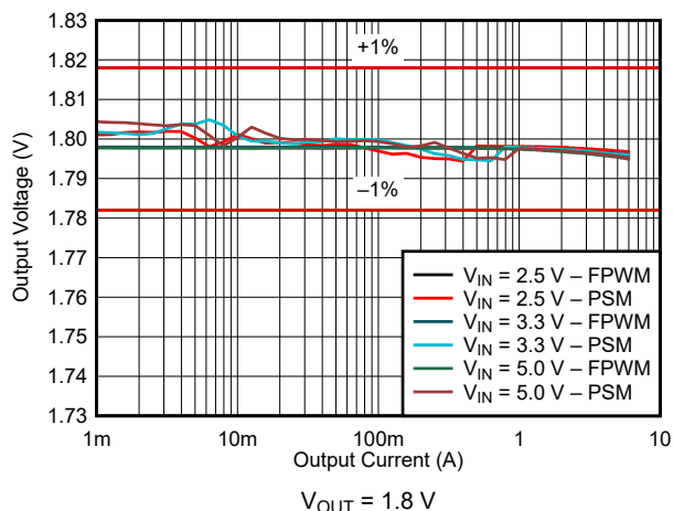
Figure 9-9. Load Regulation
