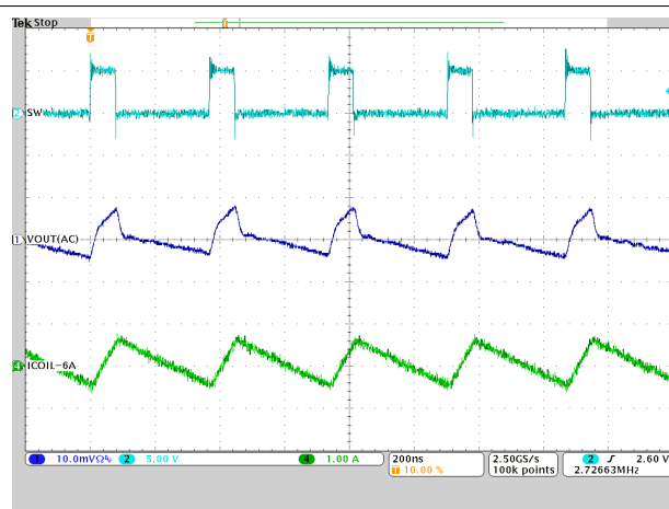
9-14. Switching Frequency
