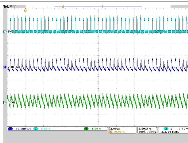
9-16. PWM Operation
