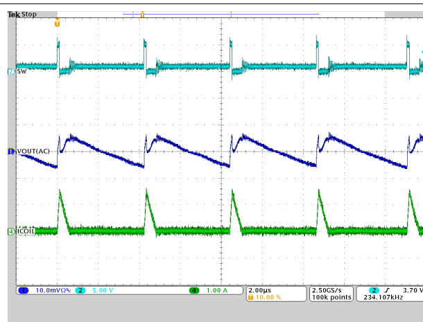
9-15. Switching Frequency
