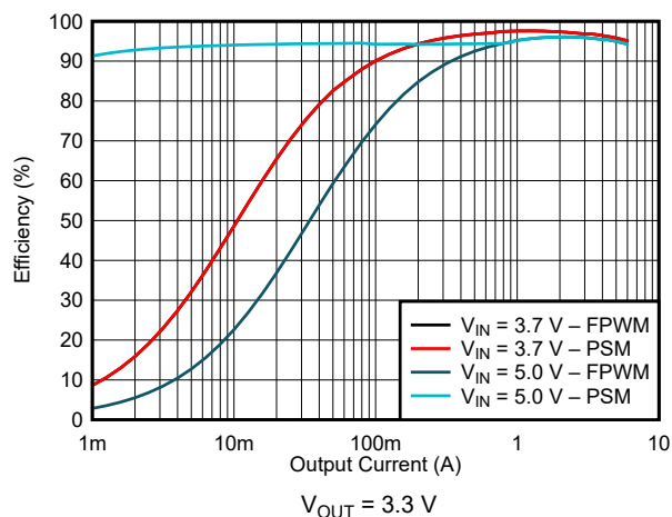
Figure 9-12. Efficiency
