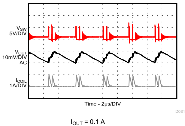
9-13. PSM Operation
