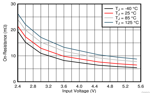
Figure 7-1. High-Side FET On-Resistance
