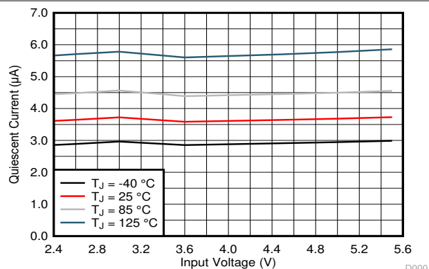
Figure 7-3. Quiescent Current
