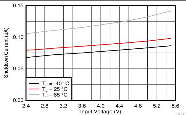
Figure 7-4. Shutdown Current
