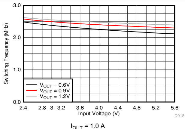
9-9. Switching Frequency
