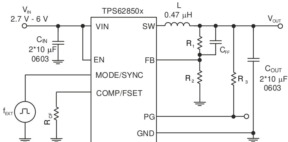
9-57. Schematic using External Synchronization
