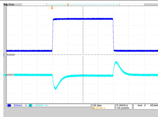
図 9-23. Load Transient Response
