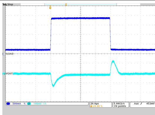
図 9-22. Load Transient Response
