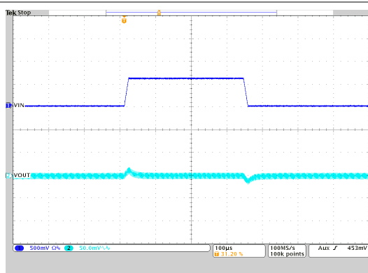
図 9-38. Line Transient Response
