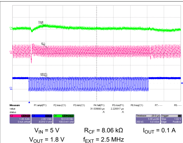
図 9-59. Switching from External Synchronization to Internal Fixed Frequency
