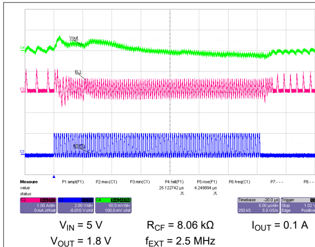
図 9-58. Switching from External Synchronization to Power-Save Mode (PFM)
