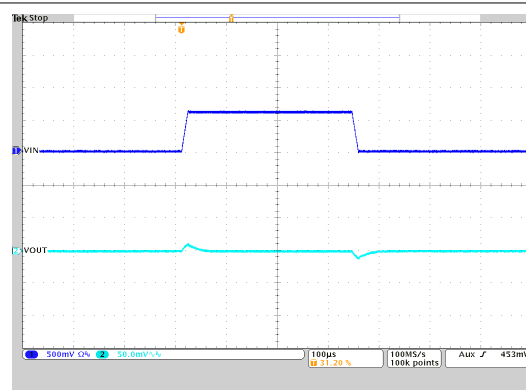
図 9-39. Line Transient Response
