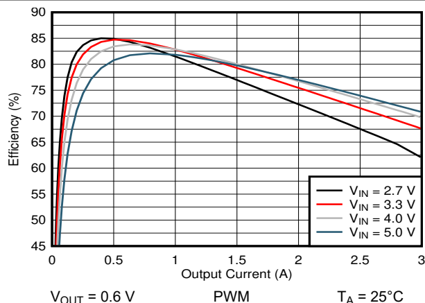
9-9. Efficiency Versus Output Current
