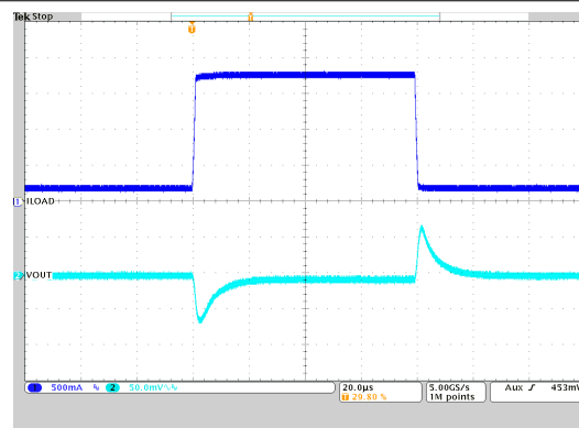
図 9-29. Load Transient Response
