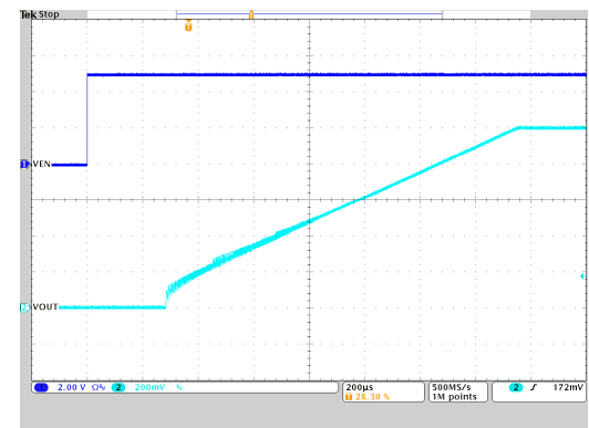
図 9-53. Start-Up Timing
