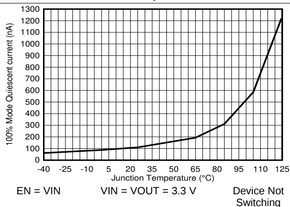
FIG 3. 100% Mode Quiescent Current ( I_{Q\_100\%\_MODE} )
