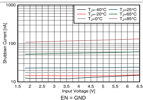
FIG 5. Shutdown Current ( I_{SD} )
