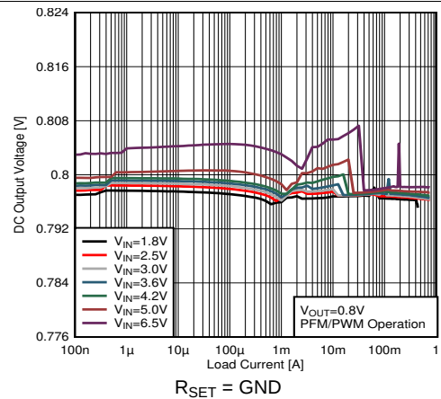
FIG 25. Output Voltage versus Load Current V OUT = 0.8 V
