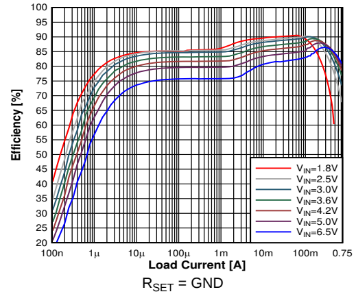
FIG 21. Efficiency Power Save Mode V OUT = 1.2 V for the DGR device
