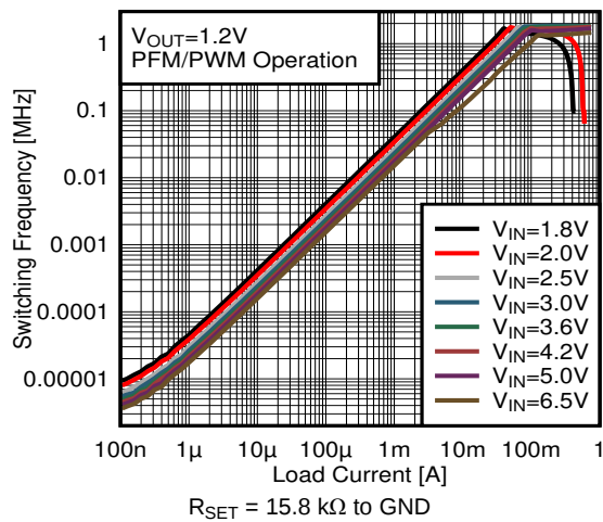
FIG 36. Switching Frequency versus Load Current V_{OUT} = 1.2\text{ V}
