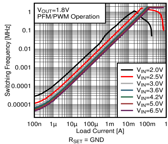
FIG 37. Switching Frequency versus Load Current V_{OUT} = 1.8\text{ V}
