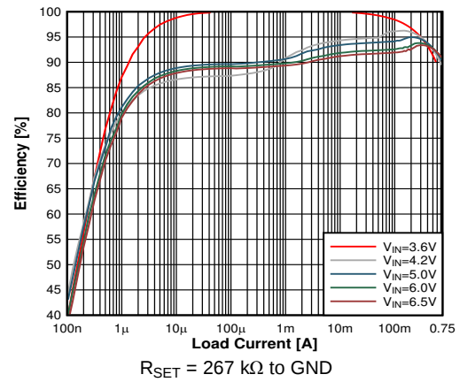
FIG 23. Efficiency Power Save Mode V OUT = 3.6 V for the DGR device
