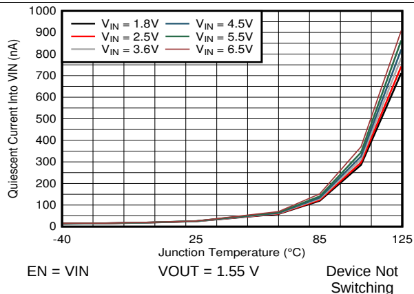
FIG 1. Quiescent Current into VIN ( I_{Q\_VIN} )
