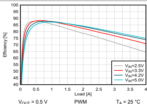
図 8-14. Efficiency versus Output Current
