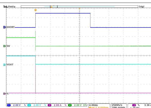
8-46. Latch-off Short-Circuit Protection
