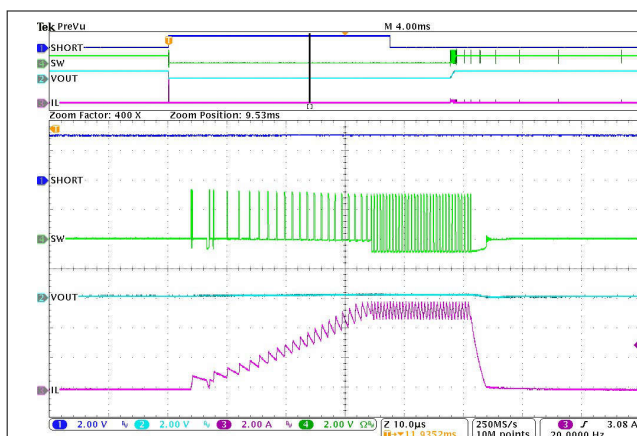
8-45. HICCUP Short-Circuit Protection (Zoom In - Second Hiccup)
