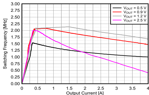
8-27. Switching Frequency versus Output Current
