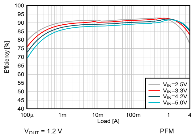
図 8-9. Efficiency versus Output Current
