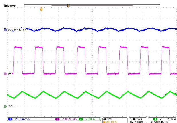
8-31. Output Voltage Ripple
