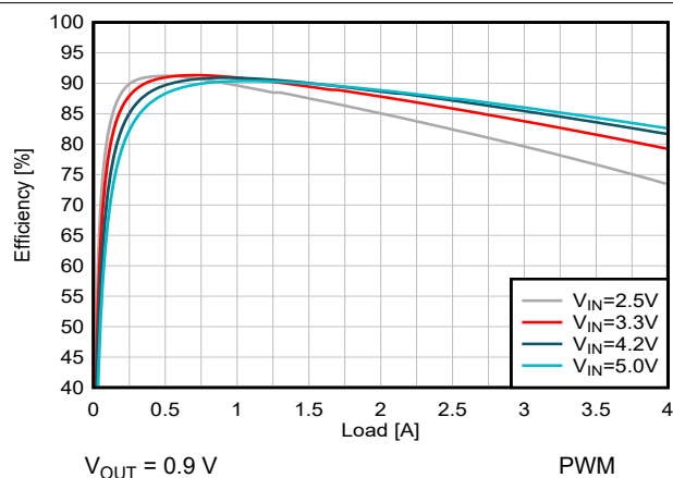
図 8-12. Efficiency versus Output Current
