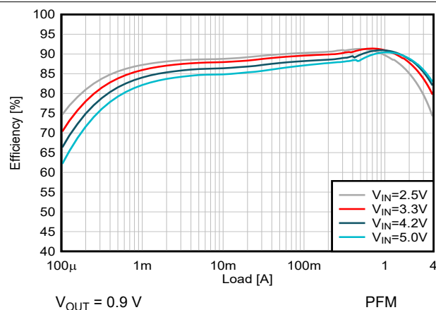
図 8-11. Efficiency versus Output Current
