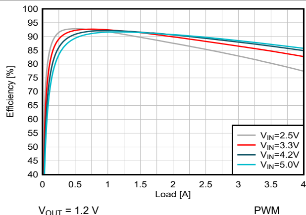
図 8-10. Efficiency versus Output Current
