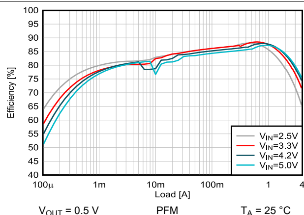
図 8-13. Efficiency versus Output Current
