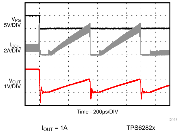
図 8-47. HICCUP Short-Circuit Protection
