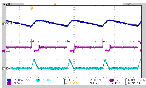
図 8-34. PSM Operation
