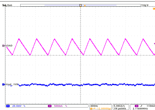
図 8-34. PSM Operation
