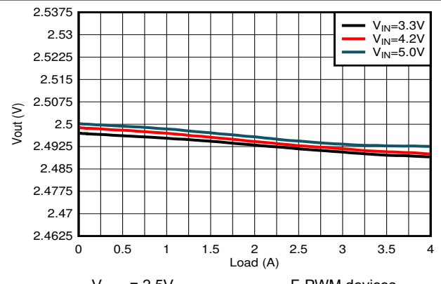
8-18. Load Regulation
