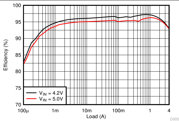
8-17. PWM Efficiency
