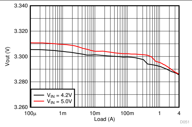
8-20. Load Regulation
