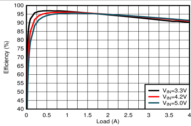
8-15. Efficiency
