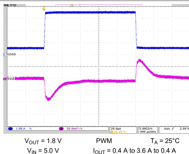
10-25. Load Transient Response
