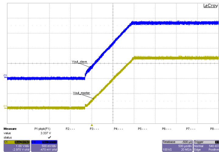
FIG 10-59. Scope Plot for Output Voltage Tracking
