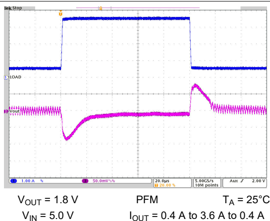
10-24. Load Transient Response
