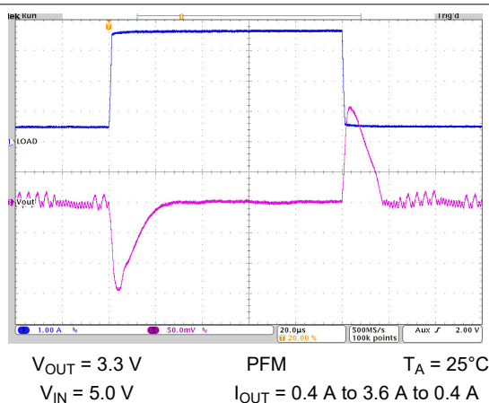
10-22. Load Transient Response
