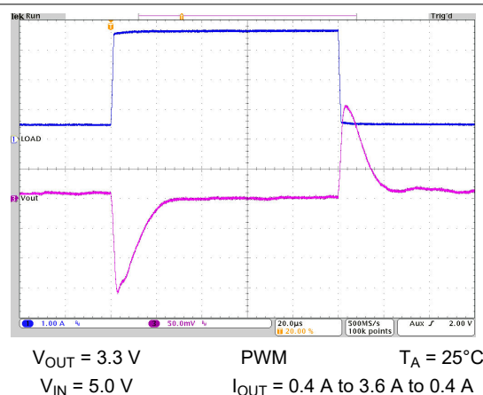
10-23. Load Transient Response
