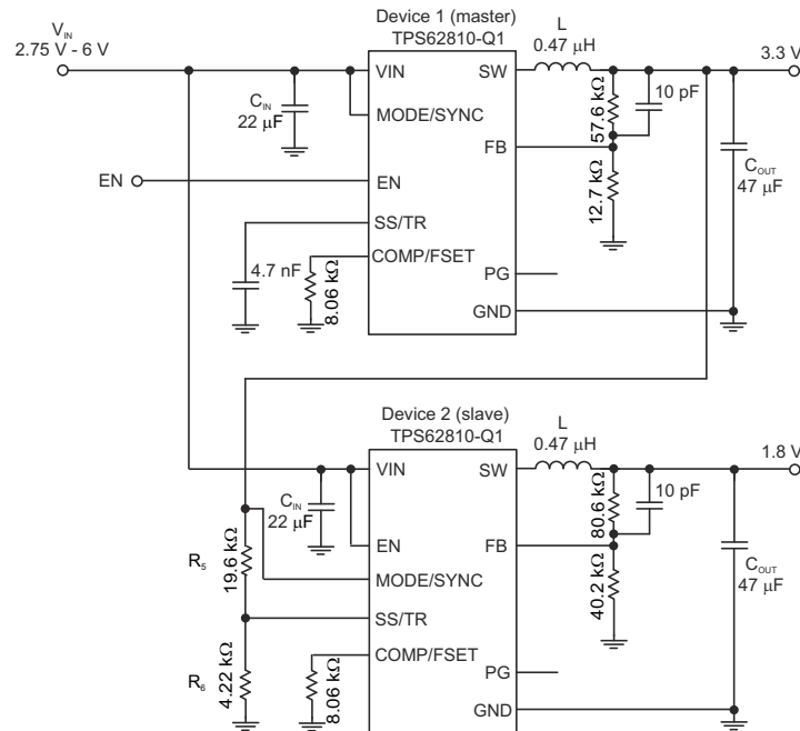
FIG 10-58. Schematic for Output Voltage Tracking
