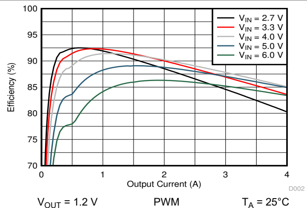
10-7. Efficiency versus Output Current
