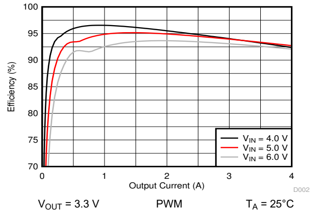
10-3. Efficiency versus Output Current
