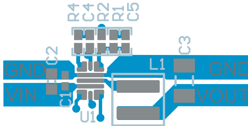
FIG 10-63. Example Layout
