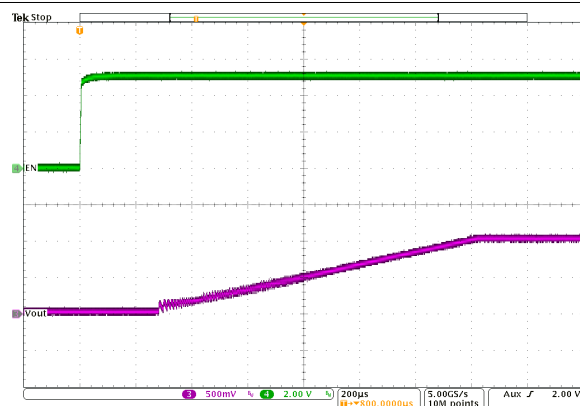
10-53. Start-Up Timing
