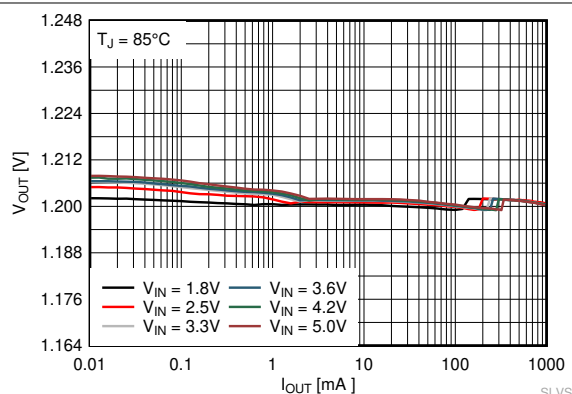
TPS62801 VSEL/MODE = GND V OUT = 1.2 V PFM/PWM モード T J = 85°C
