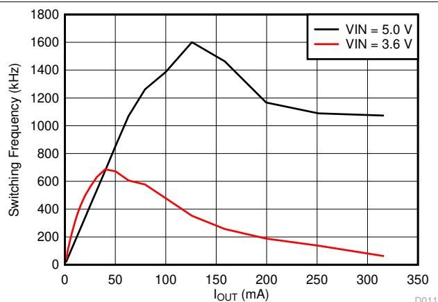
9-9. Switching Frequency vs Load Current V_{OUT} = 3.3\text{ V}
