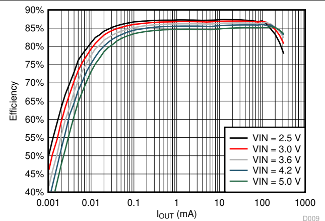
9-5. Efficiency vs Load Current; V_{OUT} = 1.8\text{ V}
