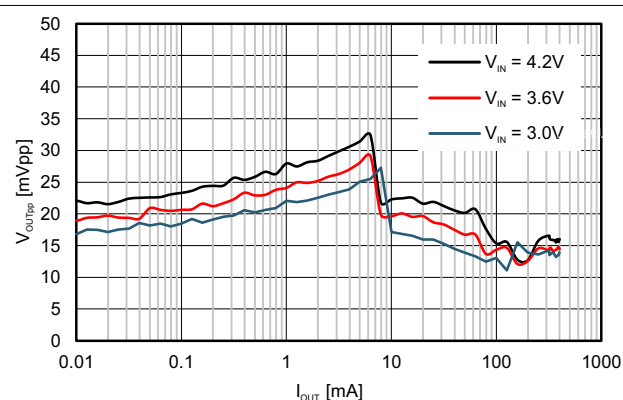
9-13. Typical Output Ripple Voltage V_{OUT} = 1.4\text{ V} TPS627431 L = 2.2\mu\text{H} C_{OUT} = 10\mu\text{F} (0402)
