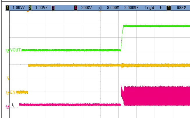
Figure 9-16. Startup Into 100 mA Electronic Load EN Delay + Soft-Start Delay
