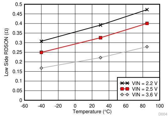
7-4. Low-side R DS(on) vs Temperature
