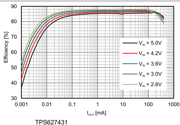
9-7. Efficiency vs Load Current; V_{OUT} = 1.4\text{ V}
