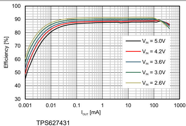
9-5. Efficiency vs Load Current; V_{OUT} = 1.9\text{ V}
