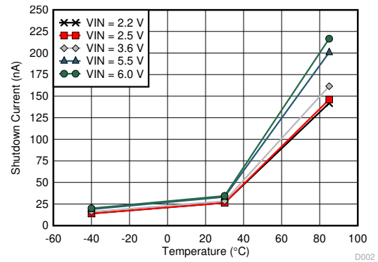
7-2. Shutdown Current I SD vs Temperature
