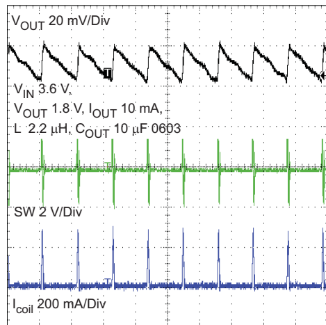
Figure 13. Typical Performance – PFM Mode
