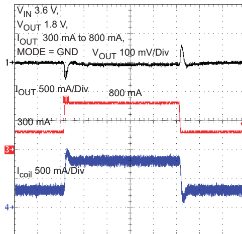
Figure 27. PWM Load Transient
