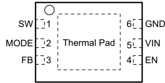
Pin Functions
