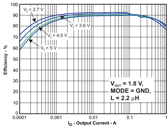
Figure 1. Efficiency vs Output Current for V_{OUT} = 1.8\text{ V} (Power-Save Mode)
