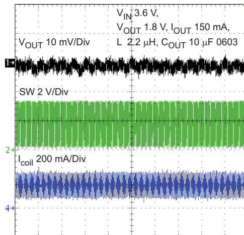
Figure 14. Typical Performance – PWM Mode
