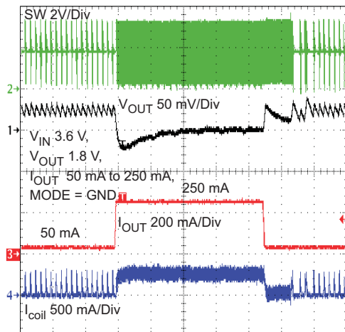
Figure 26. PFM to PWM to PFM Load Transient
