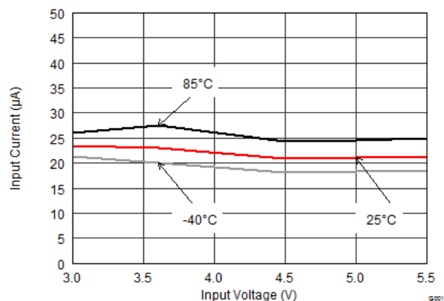
Figure 1. Quiescent Current
