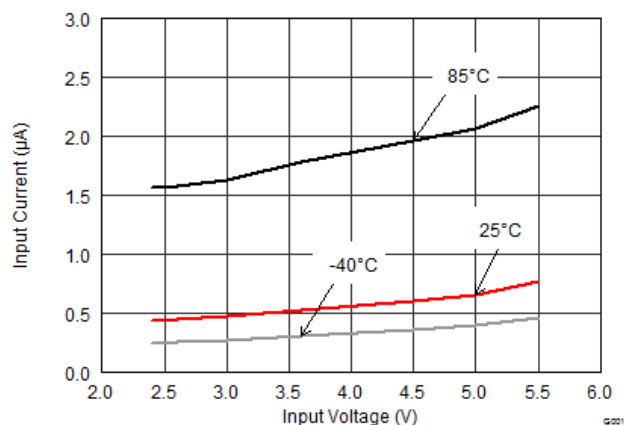
Figure 2. Shutdown Current
