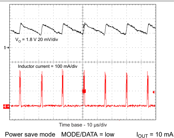
9-13. Light-Load Output-Voltage Ripple in Power-Save Mode
