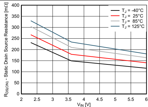
図 4. Low Side Switch Static Drain-Source On-State Resistance vs Input Voltage
