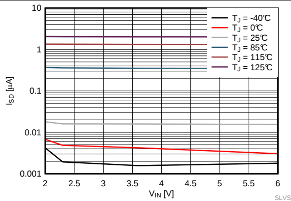
図 1. Shutdown Current vs Input Voltage
