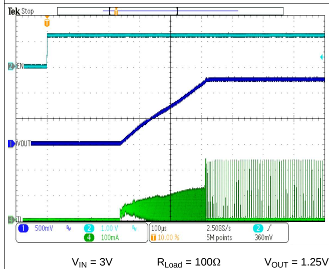
图 12. Start-Up Timing
