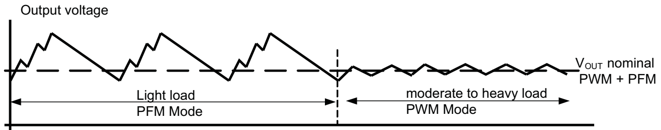
FIG 5. Power Save Mode
