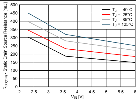
図 3. High Side Switch Static Drain-Source On-State Resistance vs Input Voltage
