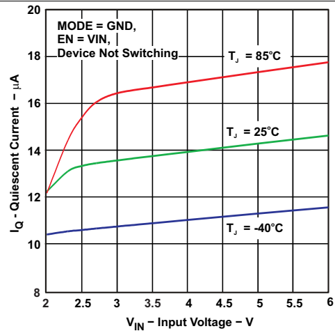
図 2. Quiescent Current vs Input Voltage
