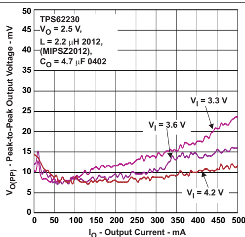
图 39. Output Voltage, Peak-to-Peak vs Output Current – TPS62230
