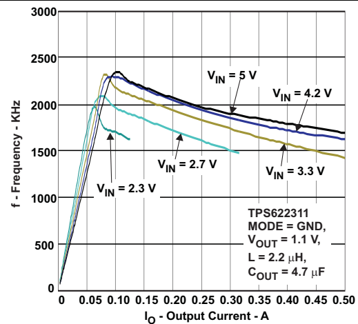
图 7. Switching Frequency vs Output Current, 1.1-V Output Voltage, PFM Mode – TPS622311
