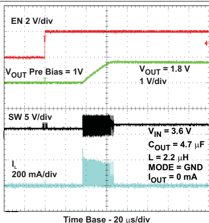
图 33. Start-Up in 1-V Prebiased Output – TPS62231
