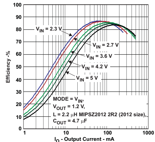
图 9. Efficiency Forced PWM Mode, 1.2-V Output Voltage – TPS62232
