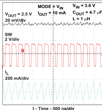
图 37. Forced PWM Mode Operation I_{\text{OUT}} = 10 \text{ mA} – TPS62230
