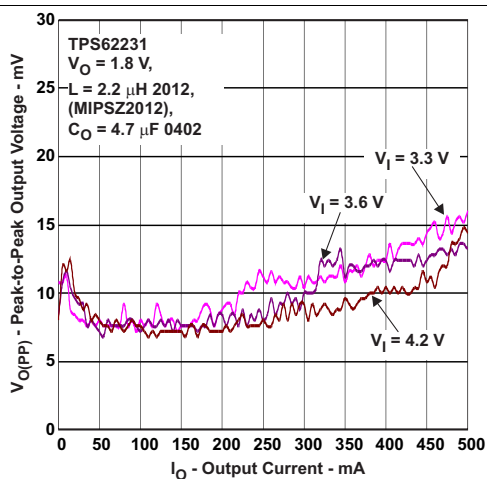
图 38. Output Voltage, Peak-to-Peak vs Output Current – TPS62231
