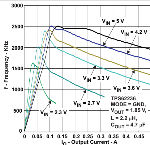
図 25. Switching Frequency vs Output Current, 1.85-V Output Voltage, PFM/PWM Mode – TPS62236
