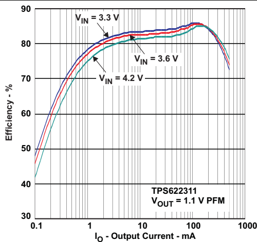
图 6. Efficiency vs I_{OUT} , PFM Mode – TPS622311
