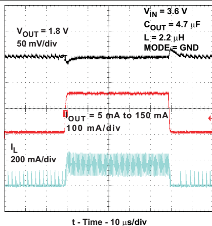
FIG 49. Load Transient Response 5 mA to 150 mA, PFM to PWM Mode, V_{OUT} 1.8 V – TPS62231
