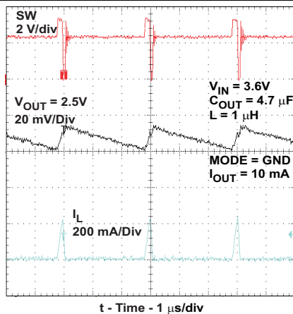
图 35. PFM Mode Operation, L = 1.0 \mu\text{H} , I_{\text{OUT}} = 10 \text{ mA} – TPS62230
