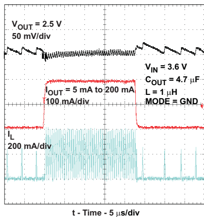
FIG 51. Load Transient Response 5 mA to 200 mA, PFM to PWM Mode, V_{OUT} 2.5 V – TPS62230
