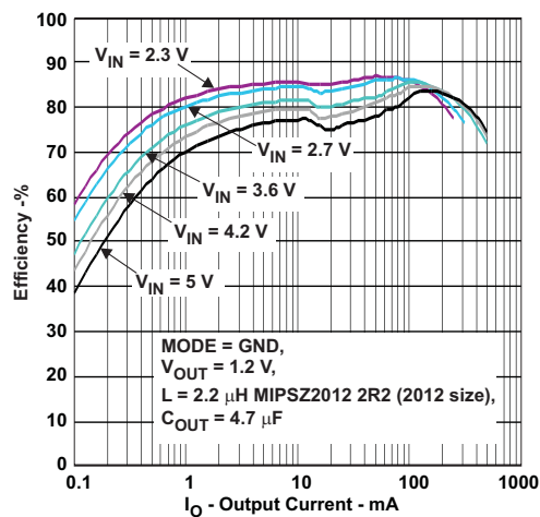
图 8. Efficiency PFM / PWM Mode, 1.2-V Output Voltage – TPS62232
