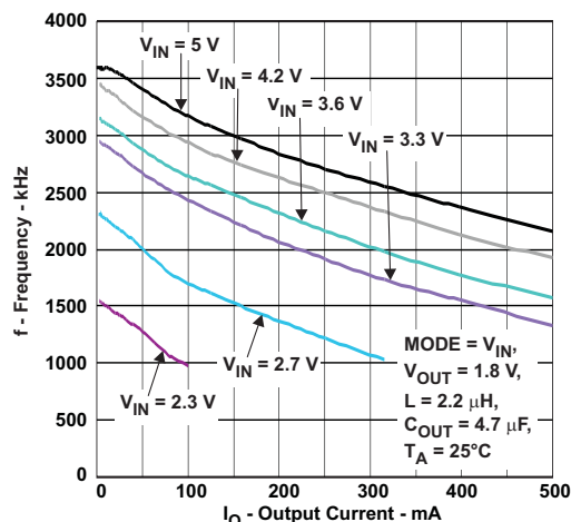
図 23. Switching Frequency vs Output Current, 1.8-V Output Voltage, Forced PWM Mode – TPS62231
