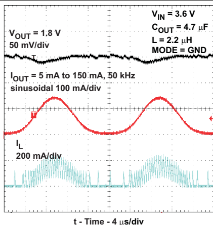
FIG 46. AC – Load Regulation Performance 1.8-V V_{OUT} , PFM Mode – TPS62231
