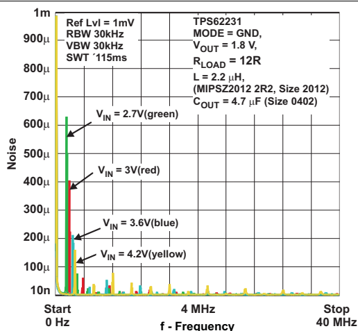
FIG 41. Spurious Output Noise, 12R Load – TPS62231
