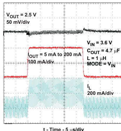
FIG 52. Load Transient Response 5 mA to 200 mA, Forced PWM Mode, V_{OUT} 2.5 V – TPS62230
