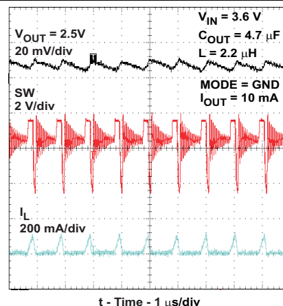
图 36. PFM Mode Operation, L = 2.2 \mu\text{H} , I_{\text{OUT}} = 10 \text{ mA} – TPS62230
