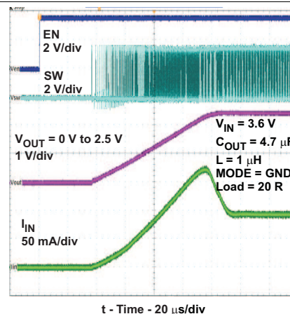
图 34. Start-Up into 20 \Omega Load, V_{OUT} 2.5 V – TPS62230
