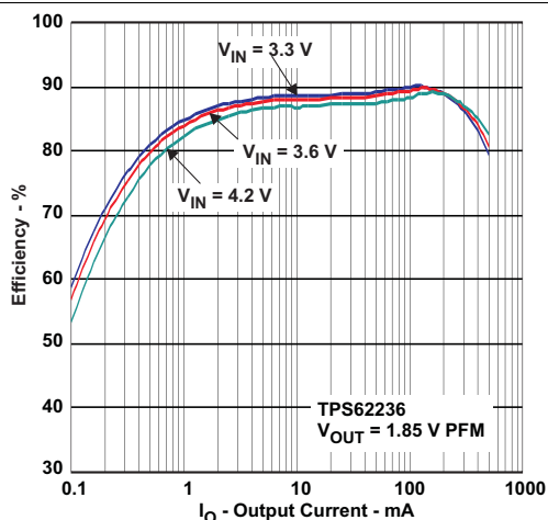
図 24. Efficiency vs I_{OUT} , PFM/PWM Mode – TPS62236
