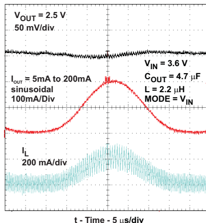
FIG 48. AC – Load Regulation Performance 2.5-V V_{OUT} , PWM Mode – TPS62230
