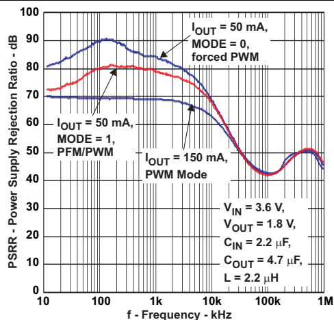
FIG 40. 1.8-V Power-Supply Rejection Ratio – TPS62231
