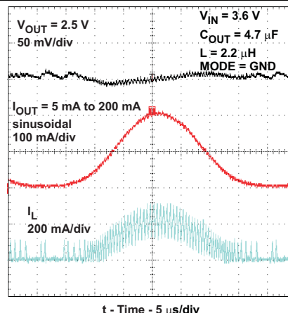
FIG 47. AC – Load Regulation Performance 2.5-V V_{OUT} , PFM Mode – TPS62230
