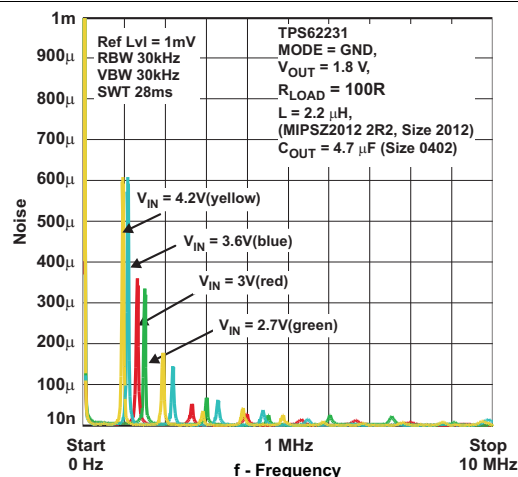
FIG 42. Spurious Output Noise, 100R Load – TPS62231
