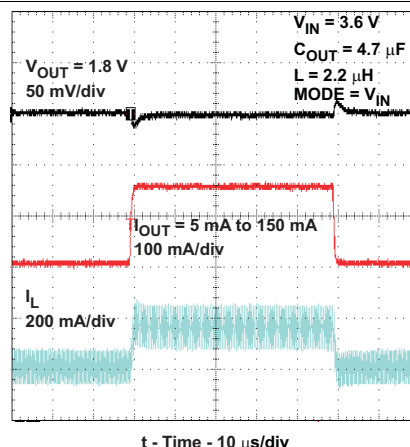
FIG 50. Load Transient Response 5 mA to 150 mA, Forced PWM Mode, V_{OUT} 1.8 V – TPS62231
