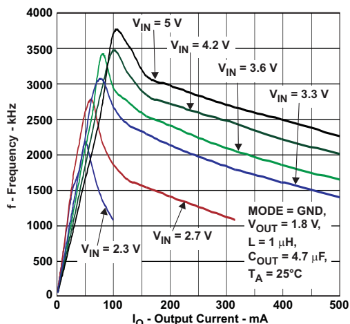
図 22. Switching Frequency vs Output Current, 1.8-V Output Voltage, PFM/PWM Mode – TPS62231
