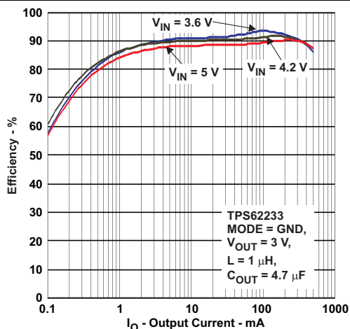
图 32. Efficiency vs I_{OUT} – TPS62233
