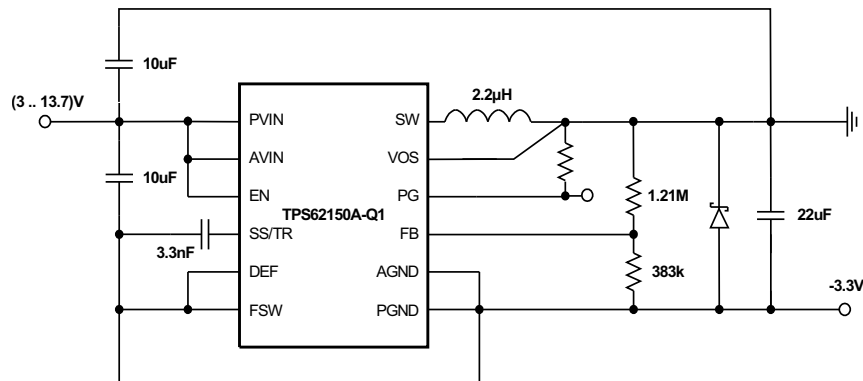
Figure 41. -3.3 V Inverting Power Supply
