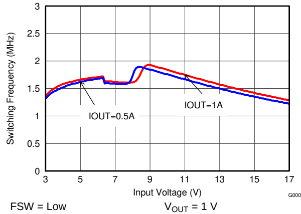
Figure 30. Switching Frequency vs Input Voltage
