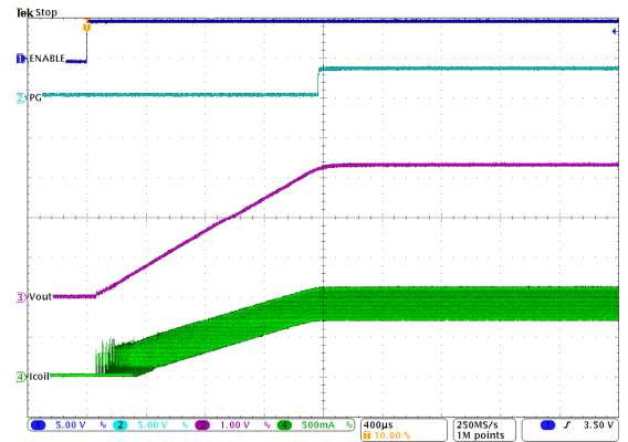
图 9-35. Start-Up Into 1 A
