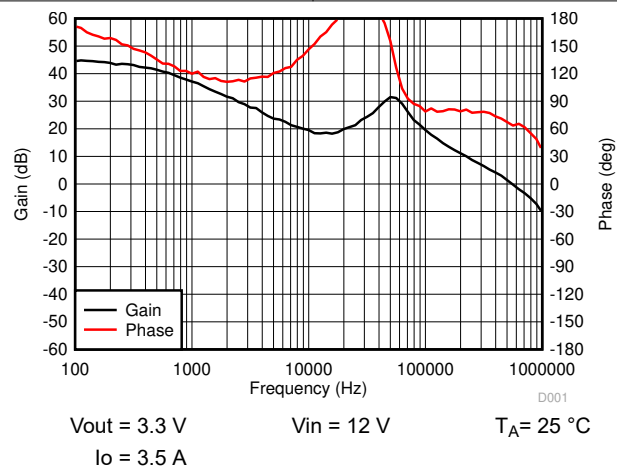
10-79. Bode Plot
