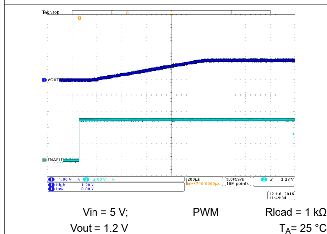
10-37. Start-Up Timing
