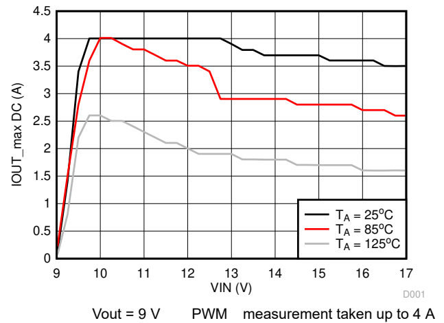
FIG 10-32. Maximum Output Current vs Input Voltage
