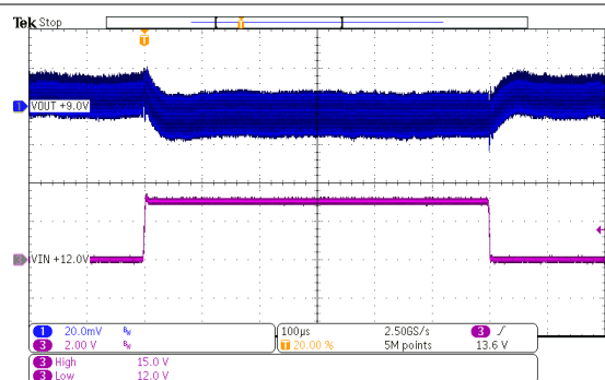
FIG 10-63. Line Transient Response
