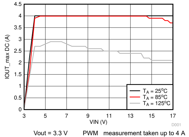
FIG 10-30. Maximum Output Current vs Input Voltage
