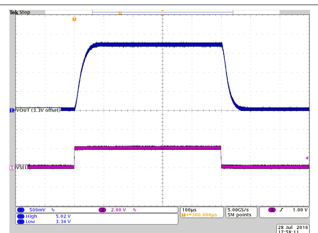
10-82. Output Voltage Change from 3.3 V to 5 V in PWM with 20 Ω load resistance
