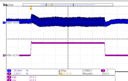
FIG 10-64. Line Transient Response
