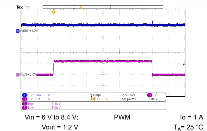
10-36. Line Transient Response
