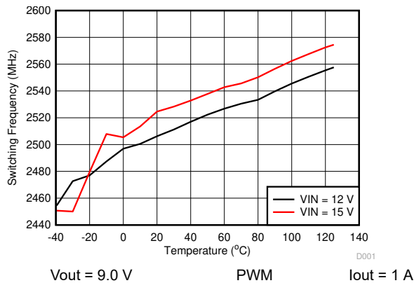
10-77. Switching Frequency vs Junction Temperature
