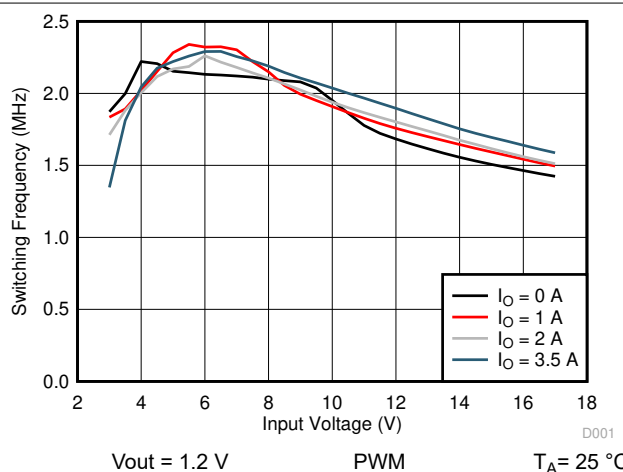
FIG 10-68. Switching Frequency vs Input Voltage
