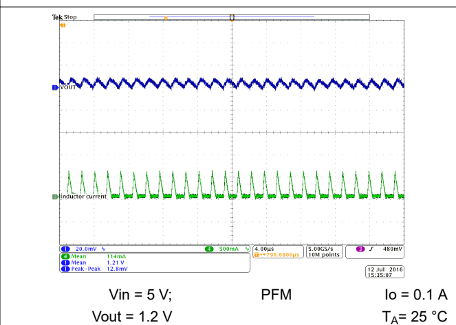
10-38. Output Voltage Ripple
