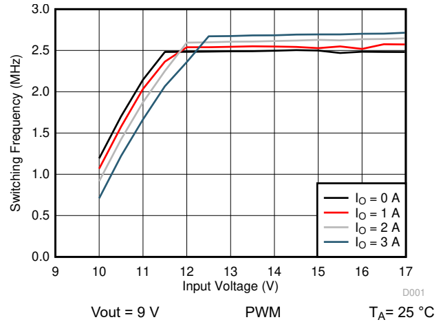
10-76. Switching Frequency vs Input Voltage
