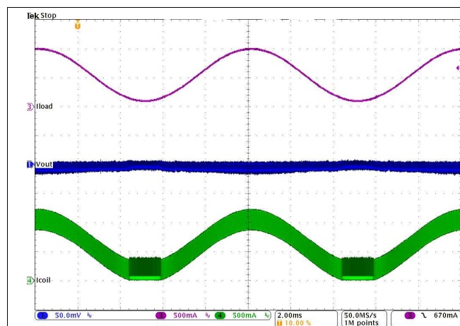
Figure 37. PWM-PSM-Transition
