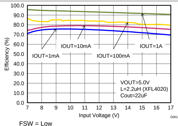
Figure 14. Efficiency vs. Input Voltage
