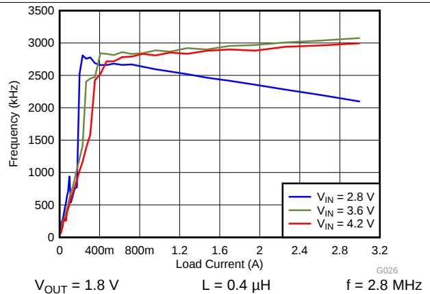
图 2. Switching Frequency vs Load Current
