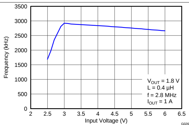
图 3. Switching Frequency vs Input Voltage
