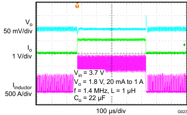
FIG 28. Load Transient Response
