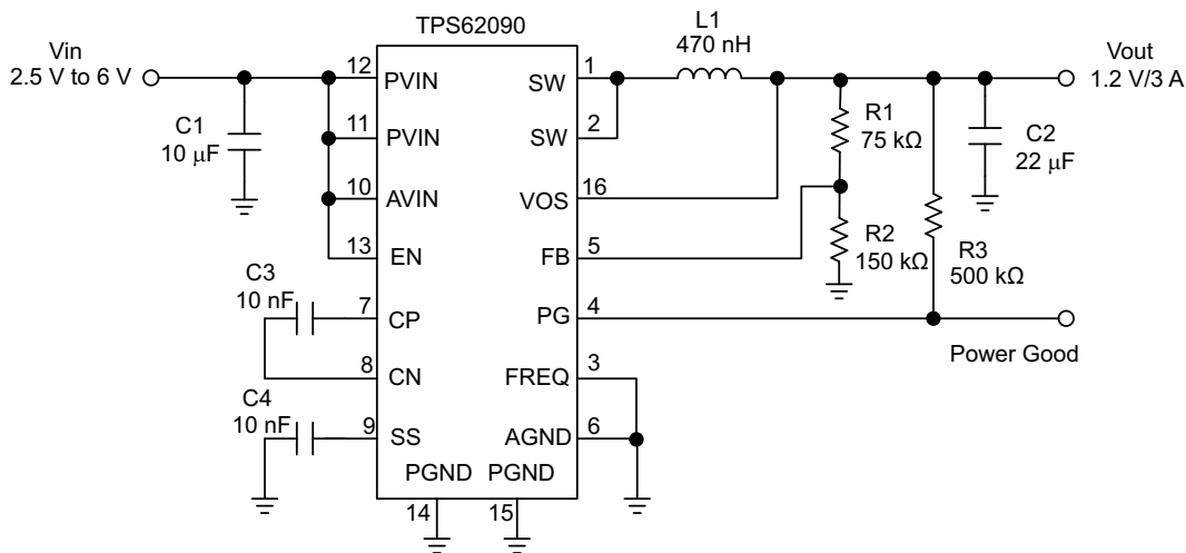
図 9. 1.2 V Adjustable Version Operating at 2.8 MHz
