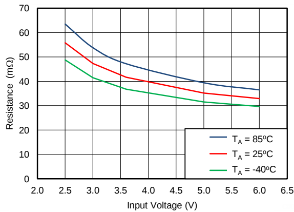
图 1. High Side FET On-Resistance vs Input Voltage
